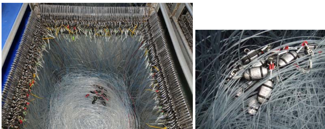
Figure 1. Branch line bin of the F/V Samurai as used in the 120 g trial (left). Clips (one end of the branch line) are attached to horizontal runners around the top of the bin and hooks (the other end of branch lines) are suspended from the clips. The branch lines joining clips and hooks are coiled in the bin along with the line weights. Some branch lines shown are fitted with sleeves adjacent to the hooks. The yellow cable ties shown were attached for the trial and are not a normal part of the fishing gear. The weights in the photo on the left are 60 g safe leads. The 120 g 'safe' leads weights used in the trial are shown in the photo on the right.
