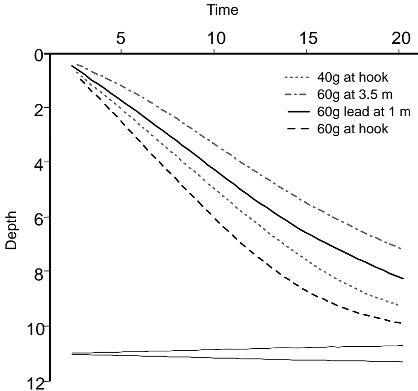
Figure 2. Average sink profiles of the two weighting regimes compared in the trial and two additional regimes with potential relevance to the fishery. The 95 % confidence bounds are shown as horizontal bars at the bottom of the figure. If the difference between any two average profiles for a given time exceeds the difference between the upper and lower arms of the confidence bounds then the difference is statistically significant. N = 30 replicates for each regime.
