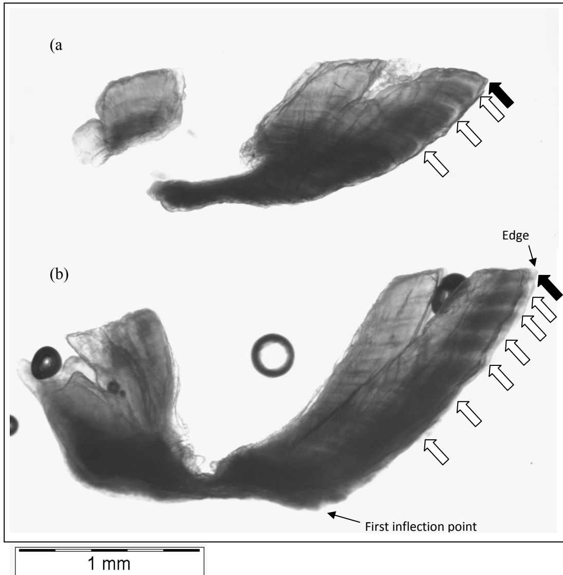
Figure 2. Images of transverse sections of sagittal otoliths under transmitted light showing clear opaque and translucent growth zones: #927 (a) and #2389 (b). Locations of the distal edges of the opaque zones counted are shown (white arrow) with a partially completed opaque zone at the margin of both otoliths (dark arrows). FL for #927 was 76 cm, and for #2389 was 89 cm.
