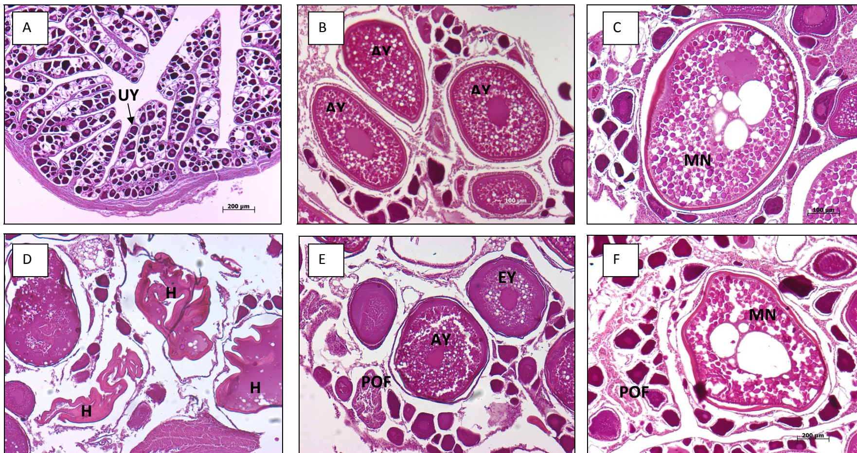
Figure 4. Histological sections of albacore ovaries showing examples of development classes, oocyte stages and postovulatory follicles. (A) unyolked oocytes in an immature ovary, (B) advanced yolked oocytes in a spawning capable ovary, (C) migratory nucleus oocyte in a spawning ovary, (D) hydrated oocytes in a spawning ovary, (E) <12 hour POF in a spawning ovary, (F) >12 hour POF in a spawning ovary. UY = unyolked, EY = early yolked, AY = advanced yolked, MN = migratory nucleus, H = hydrated, POF = postovulatory follicle.
