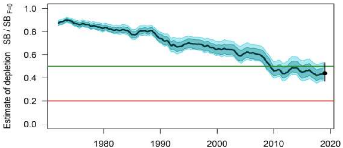
Figure SKJ-08. Plot showing the trajectories of spawning biomass depletion for the model runs included in the structural uncertainty grid weighted by the values given in Table SKJ-01. Red horizontal line indicates the agreed limit reference point, the green horizontal line indicates the interim target reference point.
