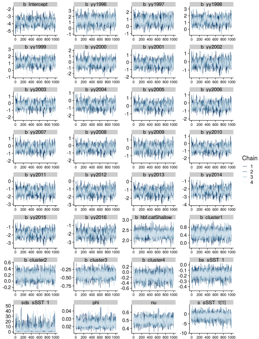
Figure A-43: Markov Chain Monte Carlo (MCMC) traces for key parameters of the observer catch rate model for the longline target fleet. Chains (4) are shown in different colours.
