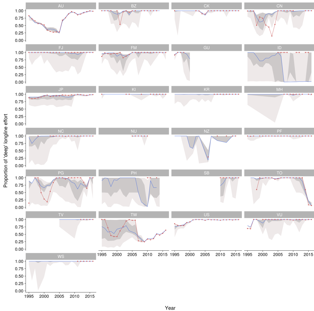
Figure 14: Prediction of the proportion of 'deep' LBEST effort over time for key longline countries in LBEST active over the assessment's region. The red line shows the observed proportion of 'deep' effort when provided and the blue line shows the prediction accounting for both observations and the random forest prediction for unobserved strata. The light and dark grey bounds show the 0.025 th - 0.975 th and 0.25 th - 0.75 th uncertainty bounds for the effort classification, also accounting for effort already provided with HBF resolution.
