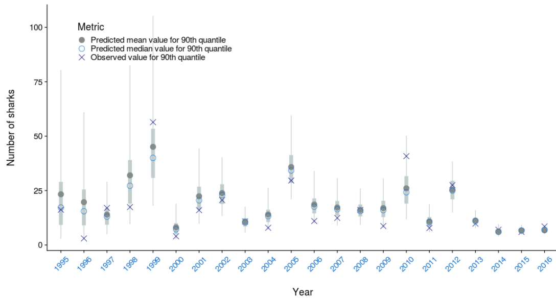
Figure A-40: Observed vs. predicted mean and median position of the 90 th quantile of oceanic whitetip shark caught by fishing event where catch > 0 by year for the longline target fleet. The median ± 25 th quantiles for the predictions is shown in grey; the whiskers cover the 2.5 - 97.5 th quantile range.
