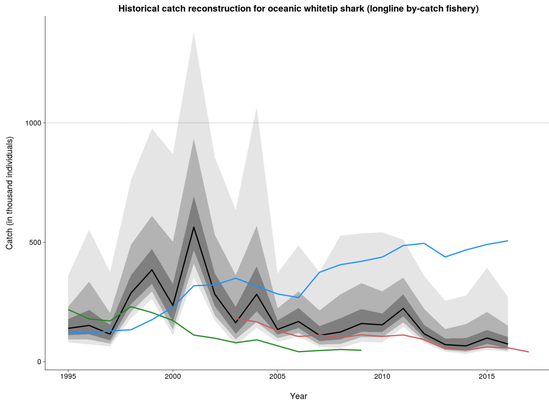
Figure 15: Median predictions of oceanic whitetip shark catch in the WCPO for the longline by-catch fleet based on a model of longline observed catch rates applied to LBEST effort. The light, dark and darker grey bounds show the 0.025 th - 0.975 th , 0.10 th - 0.90 th and 0.25 th - 0.75 th uncertainty bounds. For comparison with our estimates, the blue line shows the median prediction of historical catch based on global fin trade statistics, the red line shows the prediction of historical catch published in (Peatman et al. 2018b), and the green line shows the historical catches used for this fleet in the reference case for the 2012 assessment.
