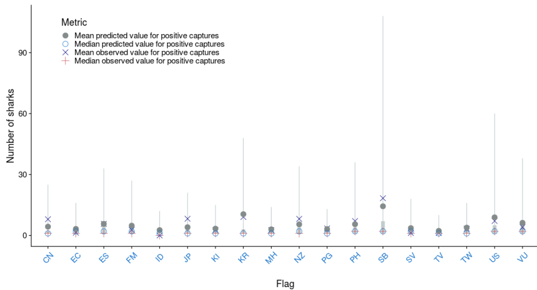
Figure A-48: Observed vs. predicted mean and median number of oceanic whitetip shark caught by fishing event where catch > 0 by flag for the observer catch rate model for the purse seine fleet. The median \pm 25 th quantiles for the predictions is shown in grey; the whiskers cover the 2.5 - 97.5 th quantile range.
