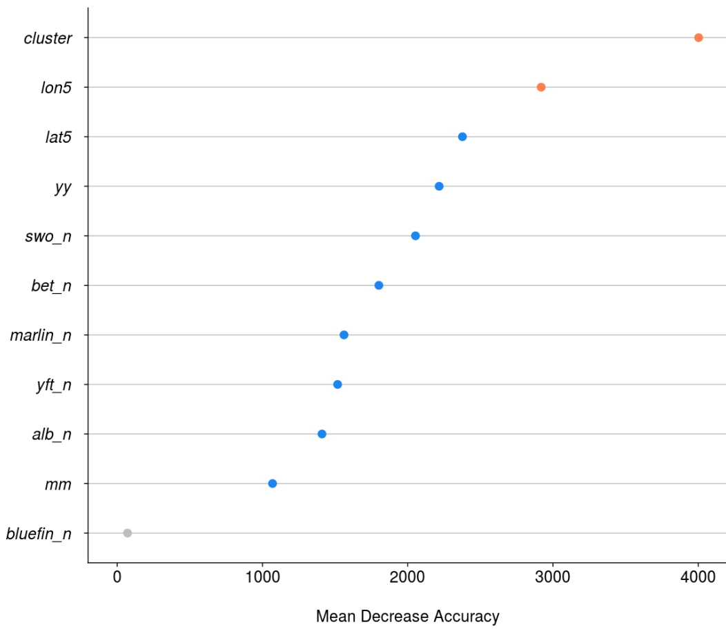
Figure 13: Importance of covariates for classification for the random forest model based on the mean decrease in the classification accuracy when the variable is excluded, ordered in decreasing abundance from top to bottom. Values highlighted in red or grey had especially high or low importance, respectively, in comparison to other covariates (blue).
