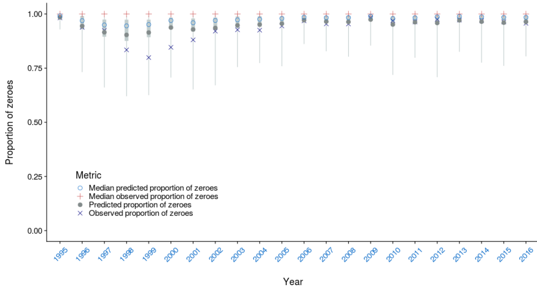
Figure A-44: Mean and median proportion of zero observed vs. predicted by fishing event for the observer catch rate model for the purse seine fleet by year. The median \pm 25 th quantiles for the predictions is shown in grey; the whiskers cover the 2.5-97.5 th quantile range.
