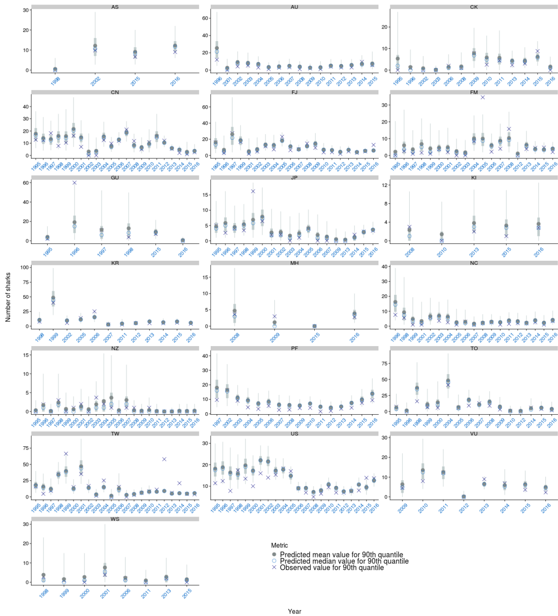
Figure A-32: Observed vs. predicted mean and median position of the 90 th quantile of oceanic whitetip shark caught by fishing event where catch > 0 by flag and year for the longline bycatch fleet. The median \pm 25 th quantiles for the predictions is shown in grey; the whiskers cover the 2.5-97.5 th quantile range.
