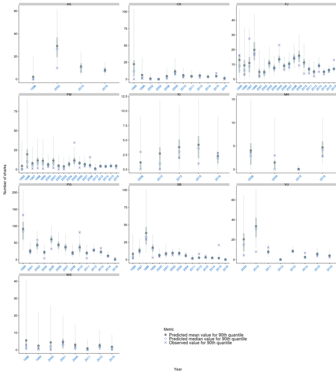
Figure A-42: Observed vs. predicted mean and median position of the 90 th quantile of oceanic whitetip shark caught by fishing event where catch > 0 by flag and year for the longline target fleet. The median \pm 25 th quantiles for the predictions is shown in grey; the whiskers cover the 2.5-97.5 th quantile range.
