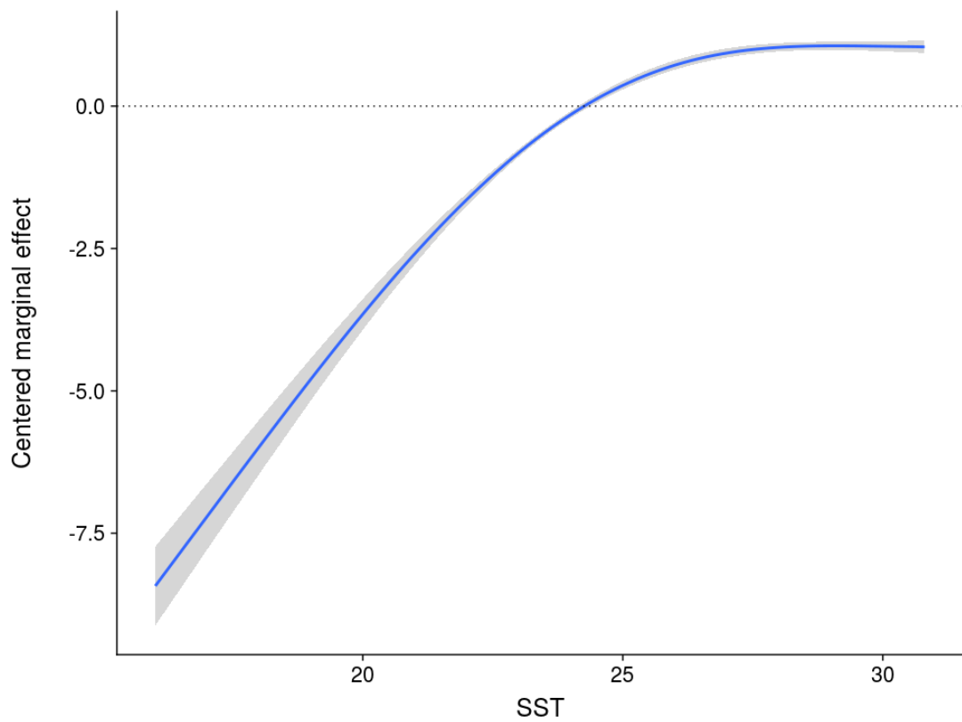
Figure 3: Predicted relationship between sea surface temperature (SST) and observed catch rates for the oceanic whitetip shark for the longline bycatch fleet, independent of other covariates.
