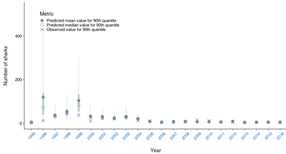
Figure A-50: Observed vs. predicted mean and median position of the 90 th quantile of oceanic whitetip shark caught by fishing event where catch > 0 by year for the purse seine fleet. The median \pm 25 th quantiles for the predictions is shown in grey; the whiskers cover the 2.5 - 97.5 th quantile range.
