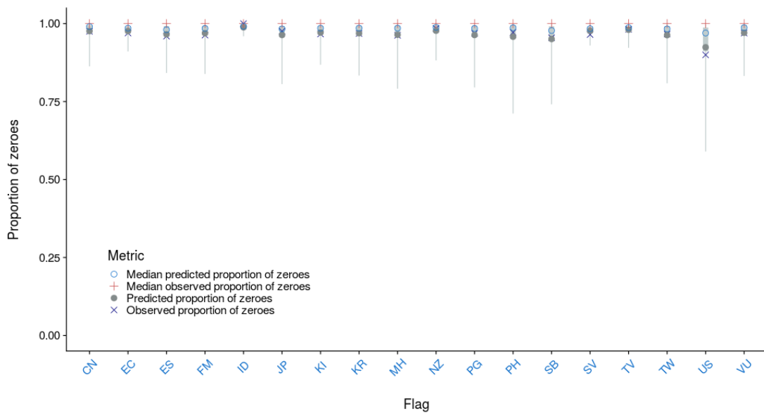
Figure A-45: Mean and median proportion of zero observed vs. predicted by fishing event for the observer catch rate model for the purse seine fleet by flag. The median \pm 25 th quantiles for the predictions is shown in grey; the whiskers cover the 2.5-97.5 th quantile range.
