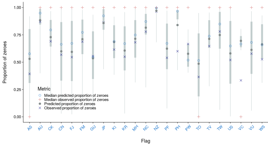
Figure A-35: Mean and median proportion of zero observed vs. predicted by fishing event for the observer catch rate model for the longline target fleet by flag. The median \pm 25 th quantiles for the predictions is shown in grey; the whiskers cover the 2.5 - 97.5 th quantile range.
