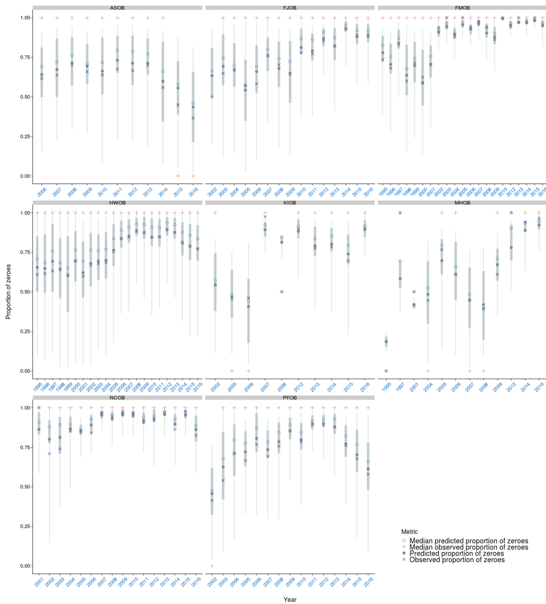
Figure A-56: Mean and median proportion of zero observed vs. predicted by fishing event for the observer catch rate model for the longline bycatch fleet by observer programme and year. The median \pm 25^{\text{th}} quantiles for the predictions is shown in grey; the whiskers cover the 2.5-97.5 th quantile range.
