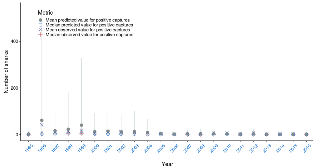
Figure A-47: Observed vs. predicted mean and median number of oceanic whitetip shark caught by fishing event where catch > 0 by year for the observer catch rate model for the purse seine fleet. The median \pm 25 th quantiles for the predictions is shown in grey; the whiskers cover the 2.5 - 97.5 th quantile range.
