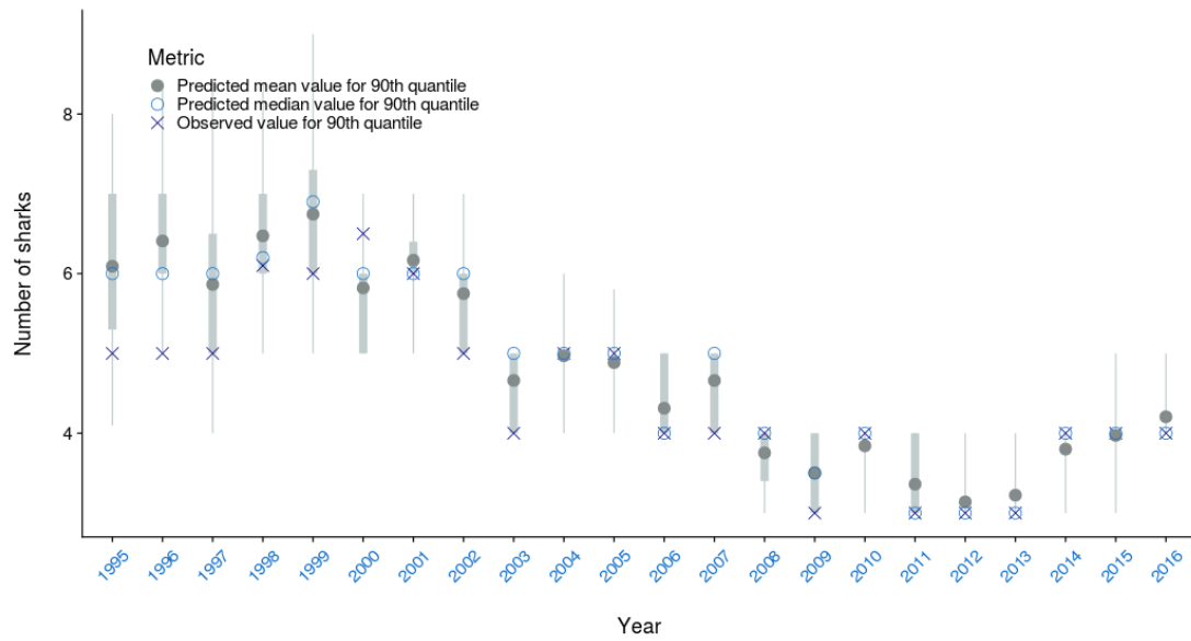
Figure A-60: Observed vs. predicted mean and median position of the 90 th quantile of oceanic whitetip shark caught by fishing event where catch > 0 by year for the longline bycatch fleet. The median ± 25 th quantiles for the predictions is shown in grey; the whiskers cover the 2.5 - 97.5 th quantile range.
