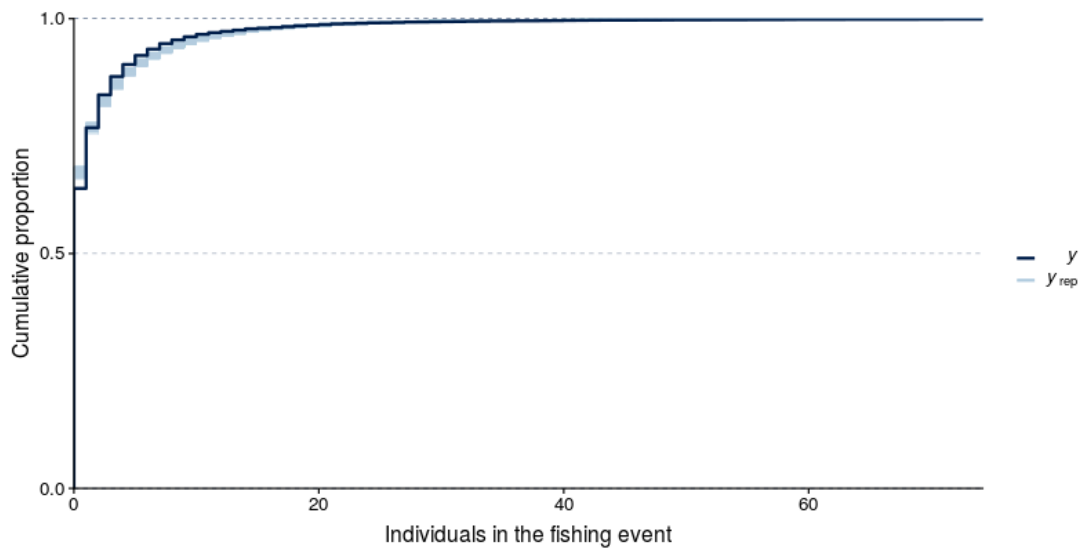
Figure 4: Posterior predictive check plot for the longline bycatch model: cumulative distribution function of the observations and draws from the model posterior showing whether the expected distribution of values for the response variable match between observations and predictions.
