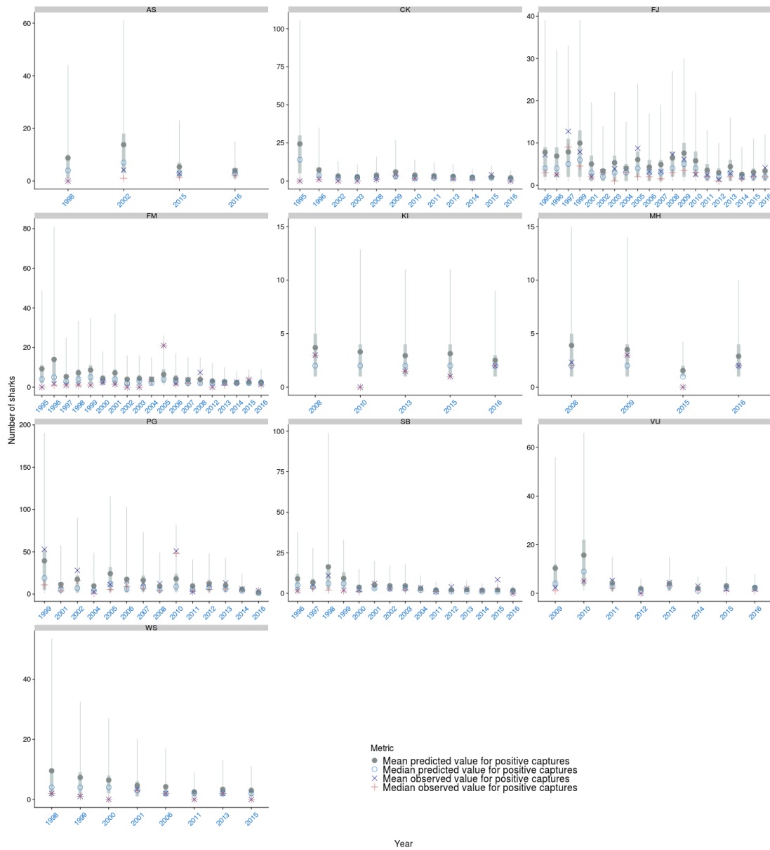
Figure A-39: Observed vs. predicted mean and median number of oceanic whitetip shark caught by fishing event where catch > 0 by flag and year for the observer catch rate model for the longline target fleet. The median \pm 25 th quantiles for the predictions is shown in grey; the whiskers cover the 2.5-97.5 th quantile range.
