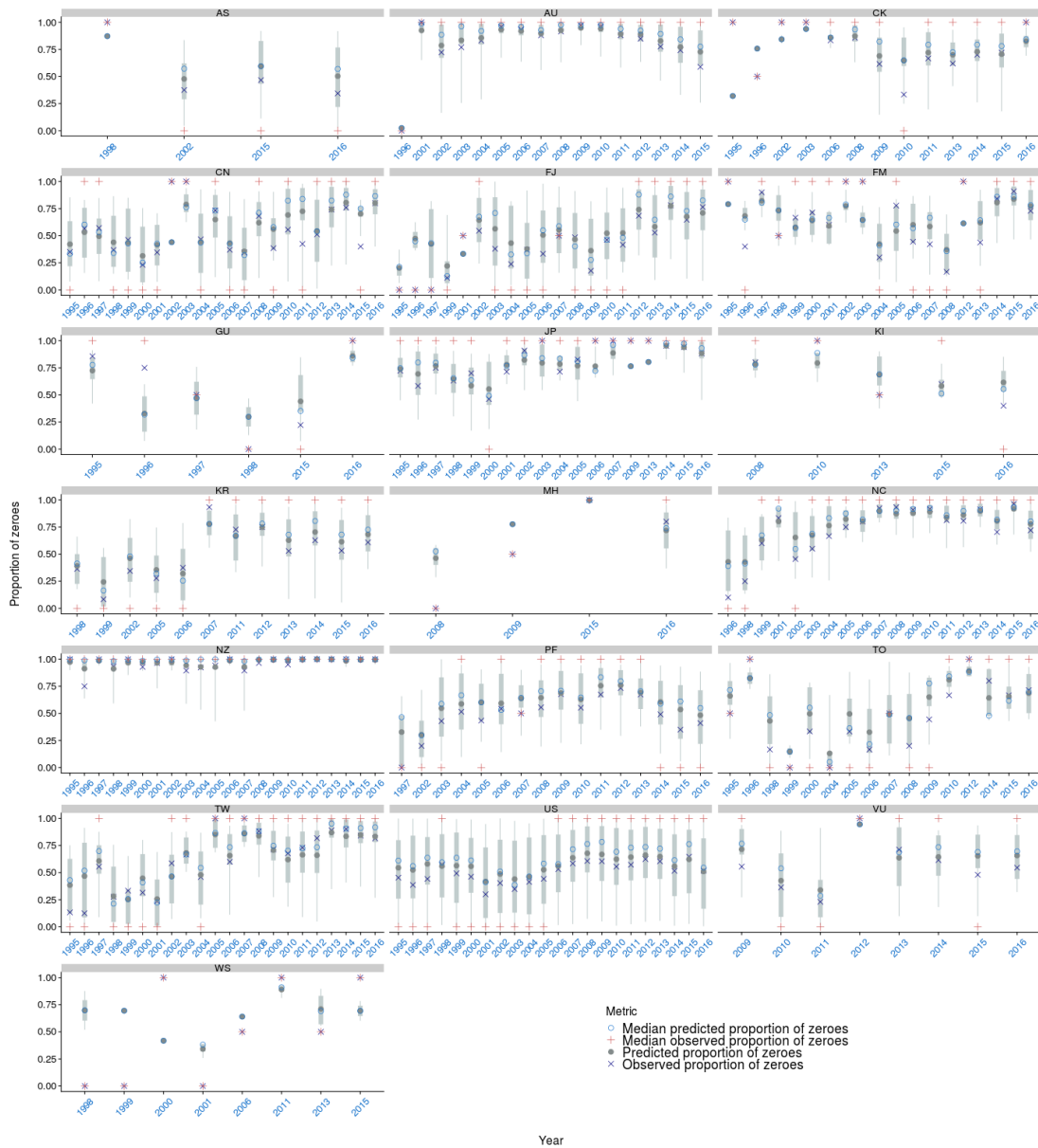
Figure A-26: Mean and median proportion of zero observed vs. predicted by fishing event for the observer catch rate model for the longline bycatch fleet by flag and year. The median \pm 25 th quantiles for the predictions is shown in grey; the whiskers cover the 2.5-97.5 th quantile range.
