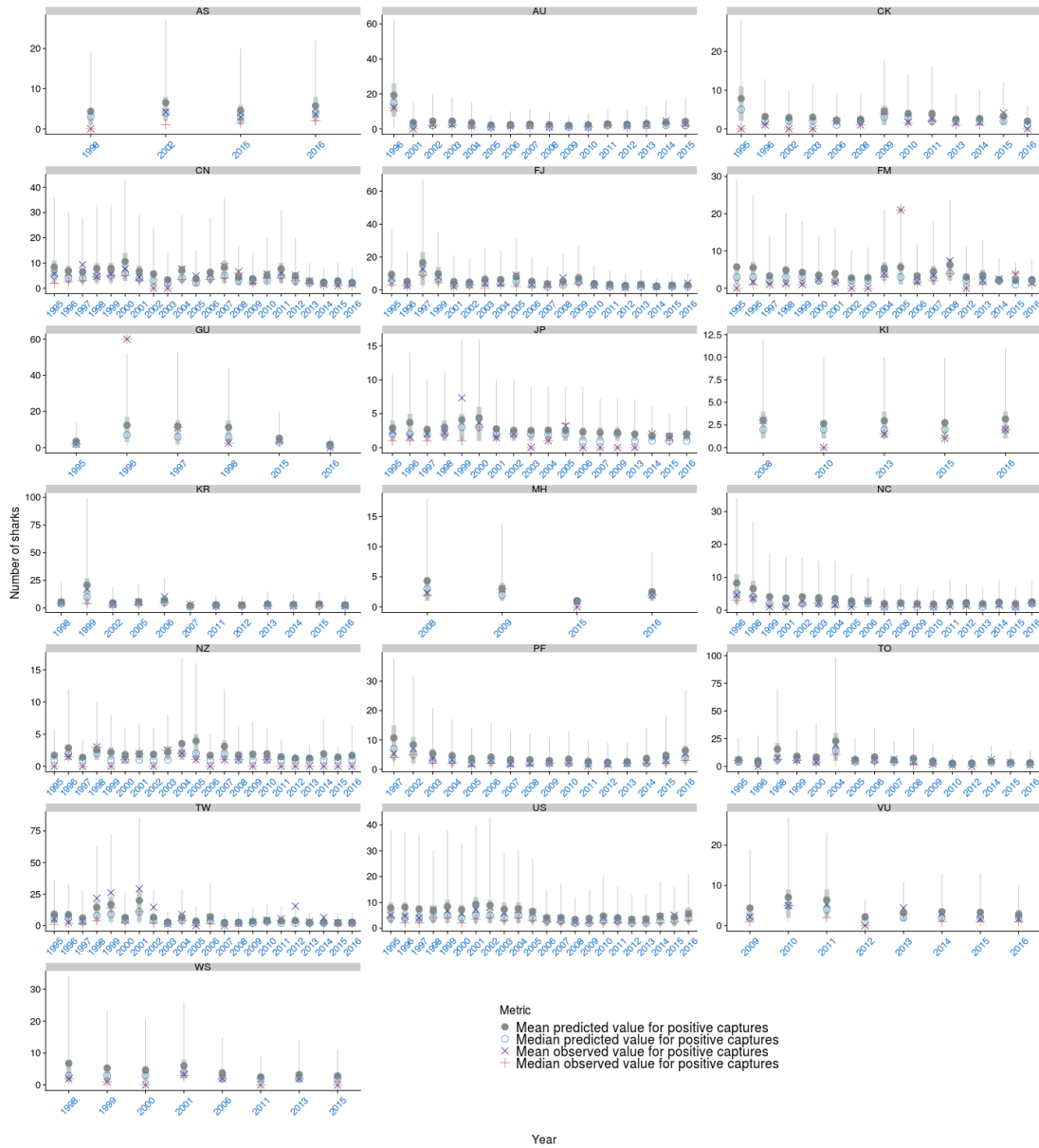
Figure A-29: Observed vs. predicted mean and median number of oceanic whitetip shark caught by fishing event where catch > 0 by flag and year for the observer catch rate model for the longline bycatch fleet. The median \pm 25 th quantiles for the predictions is shown in grey; the whiskers cover the 2.5-97.5 th quantile range.
