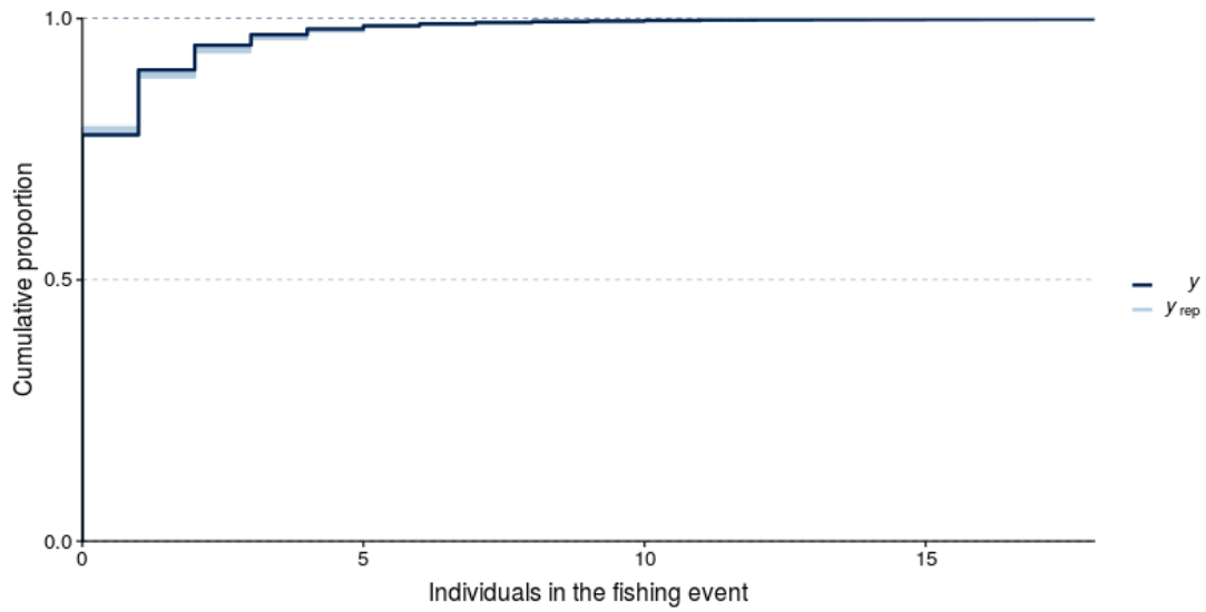
Figure 22: Posterior predictive check plot for the CPUE standardization model: cumulative distribution function of the observations and draws from the model posterior showing whether the expected distribution of values for the response variable match between observations and predictions.
