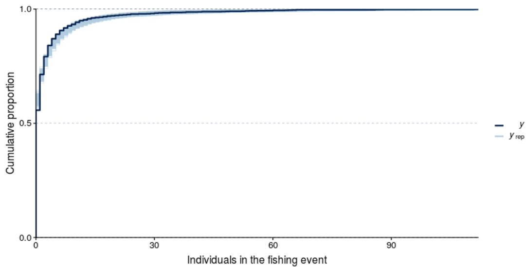
Figure 7: Posterior predictive check plot for the longline target fleet model: cumulative distribution function of the observations and draws from the model posterior showing whether the expected distribution of values for the response variable match between observations and predictions.
