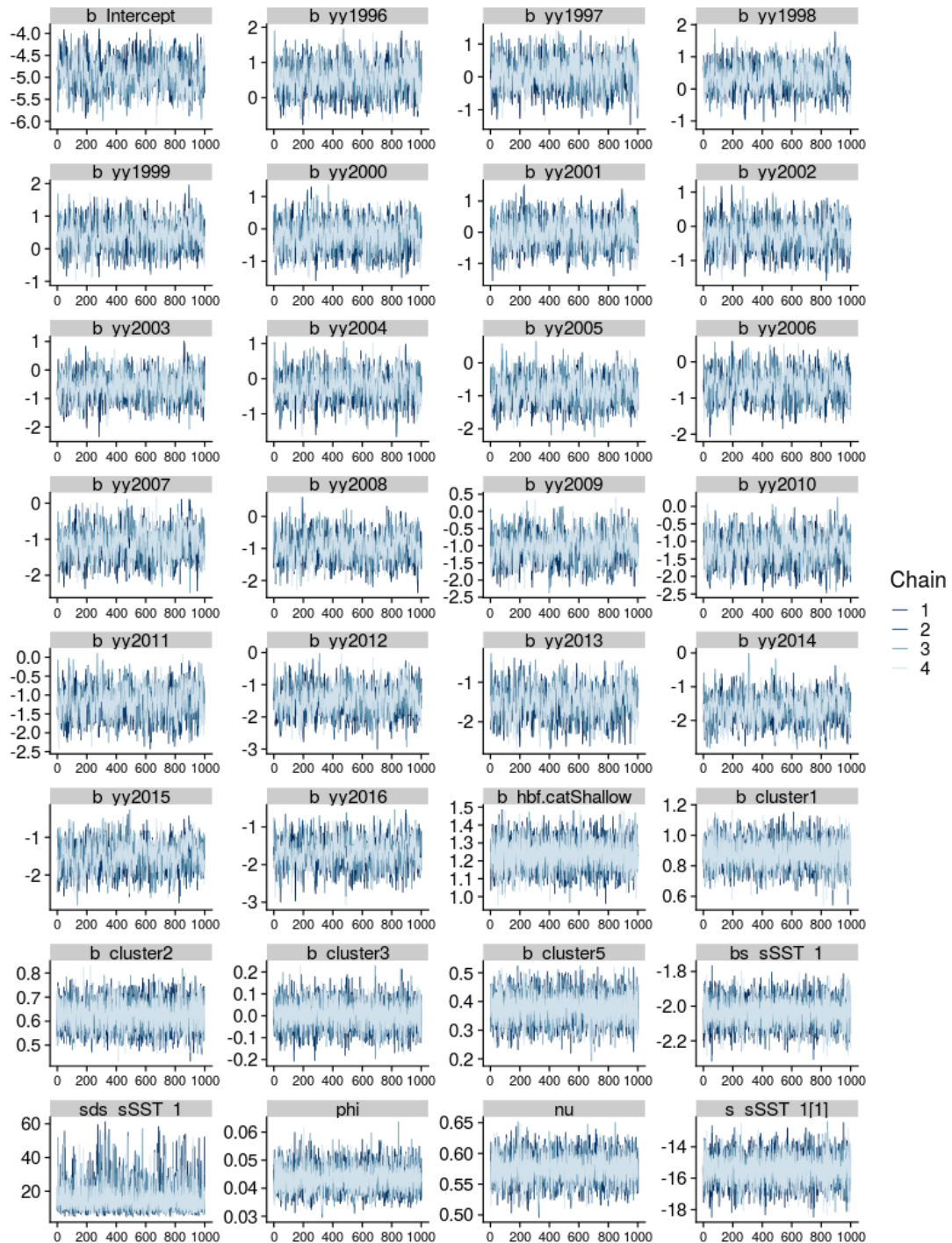
Figure A-33: Markov Chain Monte Carlo (MCMC) traces for key parameters of the observer catch rate model for the longline bycatch fleet. Chains (4) are shown in different colours.
