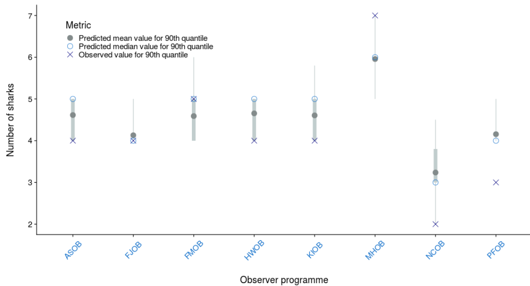
Figure A-61: Observed vs. predicted mean and median position of the 90 th quantile of oceanic whitetip shark caught by fishing event where catch > 0 by observer programme for the longline bycatch fleet. The median ± 25 th quantiles for the predictions is shown in grey; the whiskers cover the 2.5 - 97.5 th quantile range.
