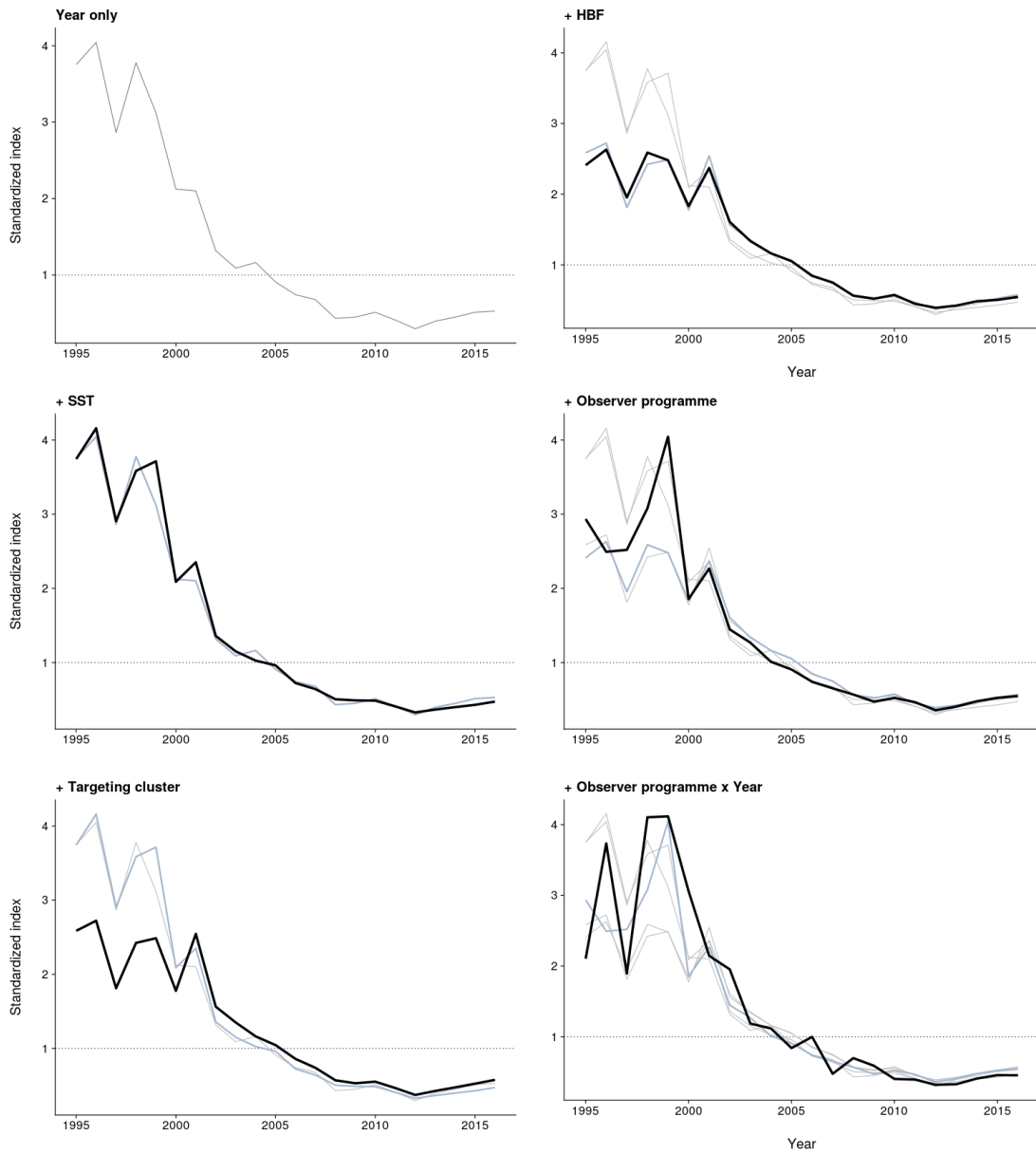
Figure 19: Stepwise plot for the CPUE standardization showing the impact on mean-centered standardized indices of gradually adding model covariates one at a time. New covariates are added from top to bottom, the updated CPUE index is shown in black and the index from the previous step is in blue. The dotted line at 1 shows the mean value for the index.
