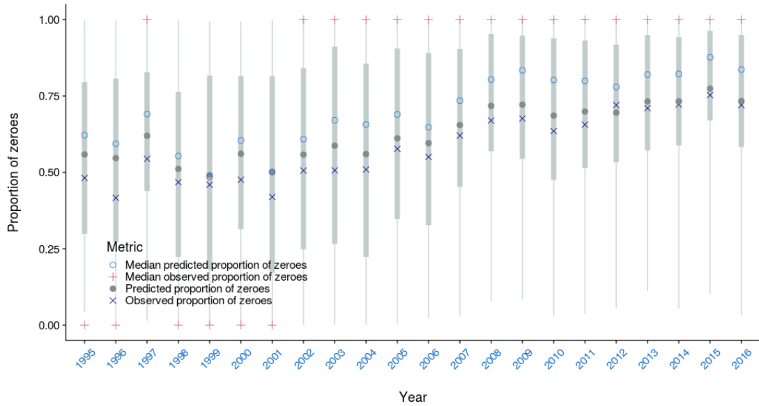
Figure A-34: Mean and median proportion of zero observed vs. predicted by fishing event for the observer catch rate model for the longline target fleet by year. The median \pm 25 th quantiles for the predictions is shown in grey; the whiskers cover the 2.5 - 97.5 th quantile range.
