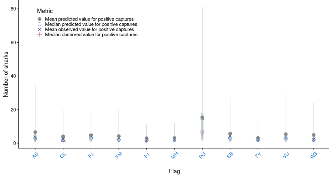
Figure A-38: Observed vs. predicted mean and median number of oceanic whitetip shark caught by fishing event where catch > 0 by flag for the observer catch rate model for the longline target fleet. The median \pm 25 th quantiles for the predictions is shown in grey; the whiskers cover the 2.5 - 97.5 th quantile range.
