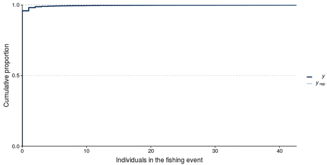
Figure 10: Posterior predictive check plot for the purse seine fleets model: cumulative distribution function of the observations and draws from the model posterior showing whether the expected distribution of values for the response variable match between observations and predictions.
