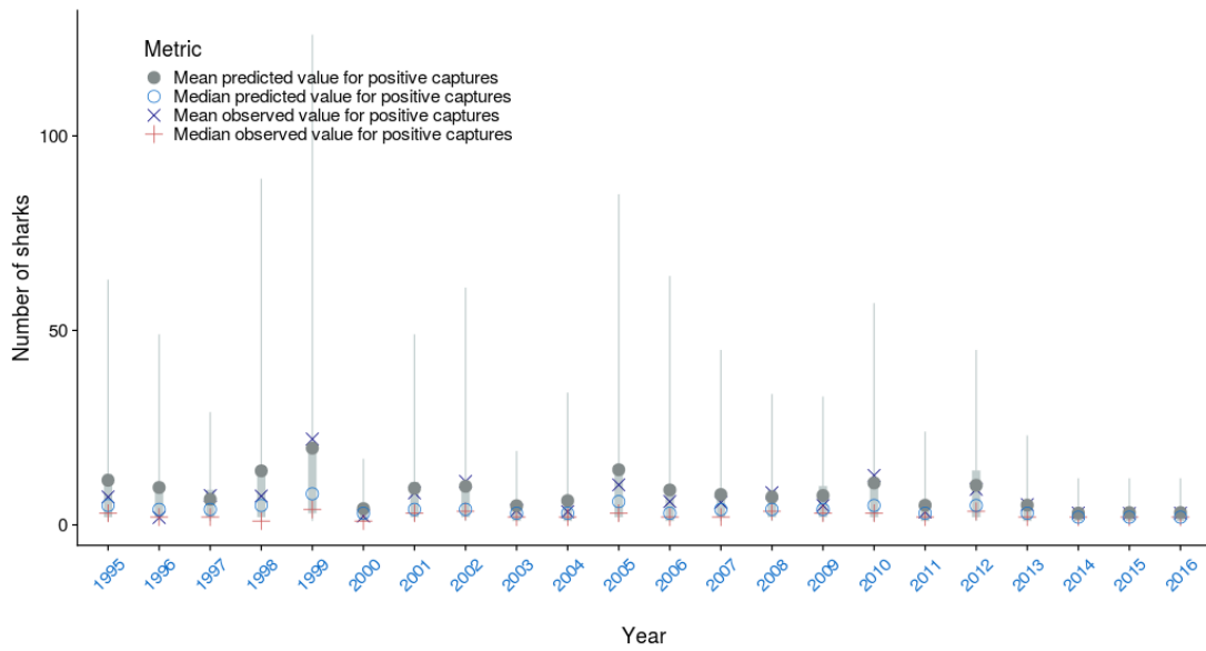
Figure A-37: Observed vs. predicted mean and median number of oceanic whitetip shark caught by fishing event where catch > 0 by year for the observer catch rate model for the longline target fleet. The median \pm 25 th quantiles for the predictions is shown in grey; the whiskers cover the 2.5 - 97.5 th quantile range.
