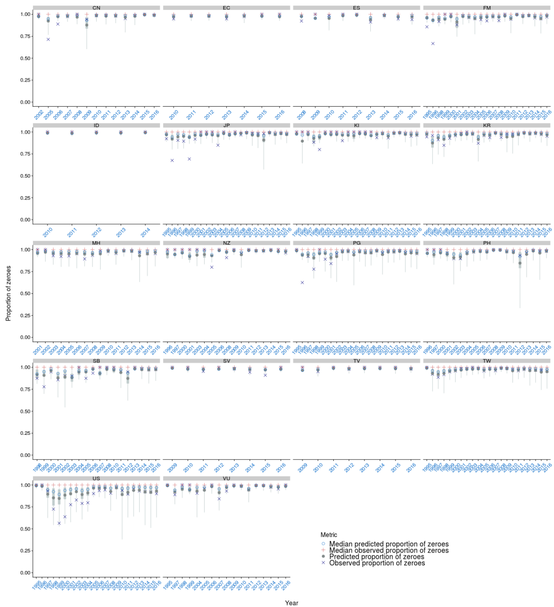
Figure A-46: Mean and median proportion of zero observed vs. predicted by fishing event for the observer catch rate model for the purse seine fleet by flag and year. The median \pm 25 th quantiles for the predictions is shown in grey; the whiskers cover the 2.5 - 97.5 th quantile range.
