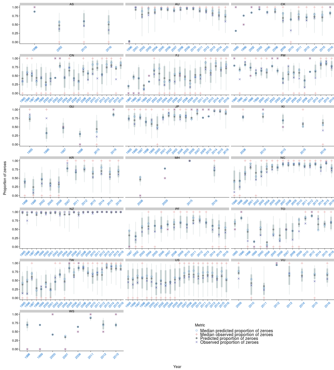
Figure A-36: Mean and median proportion of zero observed vs. predicted by fishing event for the observer catch rate model for the longline target fleet by flag and year. The median \pm 25 th quantiles for the predictions is shown in grey; the whiskers cover the 2.5-97.5 th quantile range.
