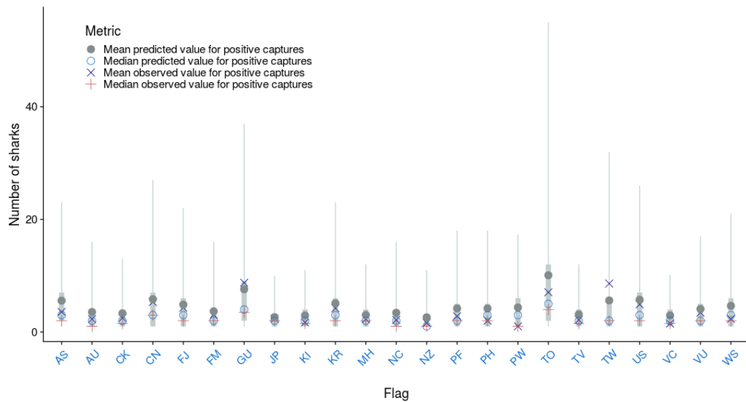
Figure A-28: Observed vs. predicted mean and median number of oceanic whitetip shark caught by fishing event where catch > 0 by flag for the observer catch rate model for the longline bycatch fleet. The median \pm 25 th quantiles for the predictions is shown in grey; the whiskers cover the 2.5-97.5 th quantile range.
