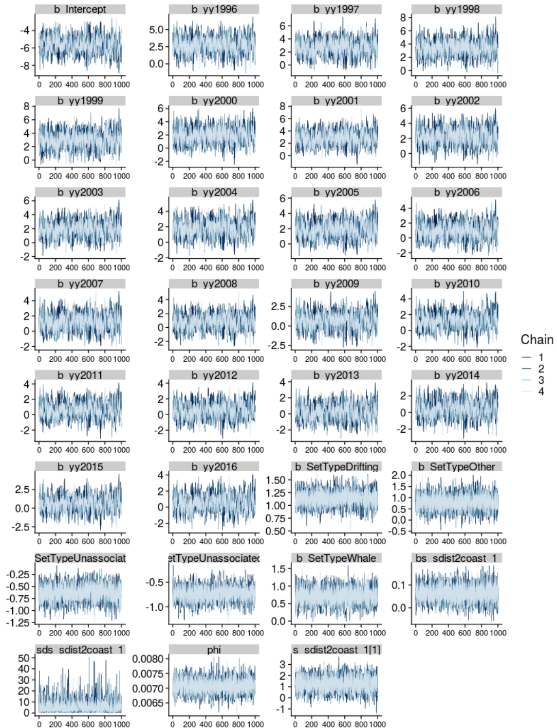
Figure A-53: Markov Chain Monte Carlo (MCMC) traces for key parameters of the observer catch rate model for the purse seine fleet. Chains (4) are shown in different colours.
