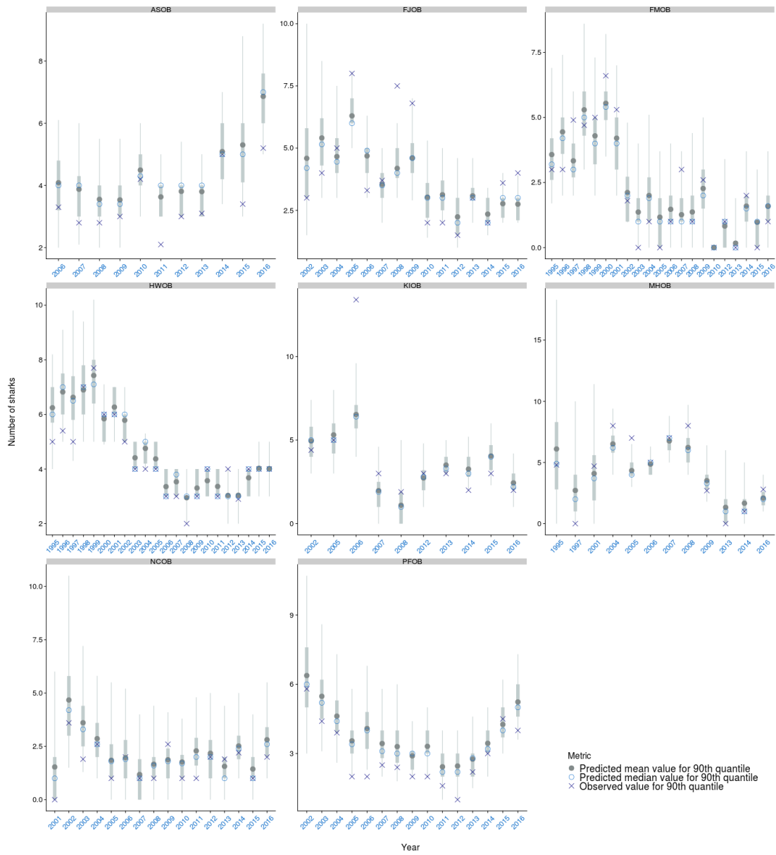
Figure A-62: Observed vs. predicted mean and median position of the 90 th quantile of oceanic whitetip shark caught by fishing event where catch > 0 by observer programme and year for the longline bycatch fleet. The median \pm 25 th quantiles for the predictions is shown in grey; the whiskers cover the 2.5-97.5 th quantile range.
