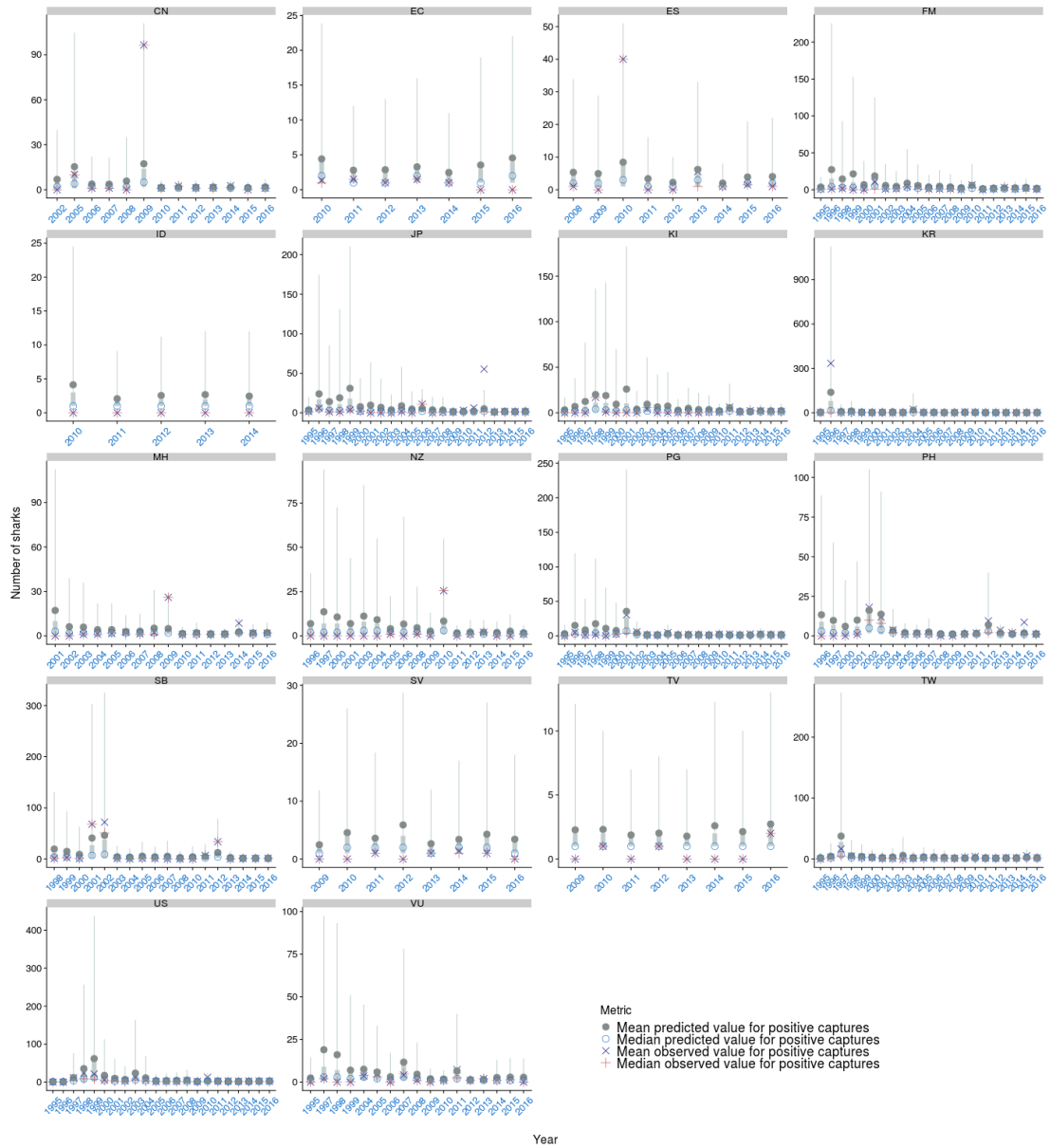
Figure A-49: Observed vs. predicted mean and median number of oceanic whitetip shark caught by fishing event where catch > 0 by flag and year for the observer catch rate model for the purse seine fleet. The median \pm 25 th quantiles for the predictions is shown in grey; the whiskers cover the 2.5-97.5 th quantile range.
