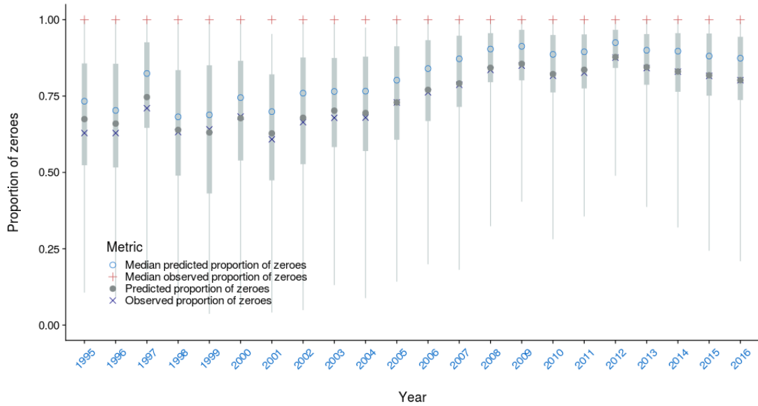
Figure A-54: Mean and median proportion of zero observed vs. predicted by fishing event for the observer catch rate model for the longline bycatch fleet by year. The median \pm 25 th quantiles for the predictions is shown in grey; the whiskers cover the 2.5 - 97.5 th quantile range.
