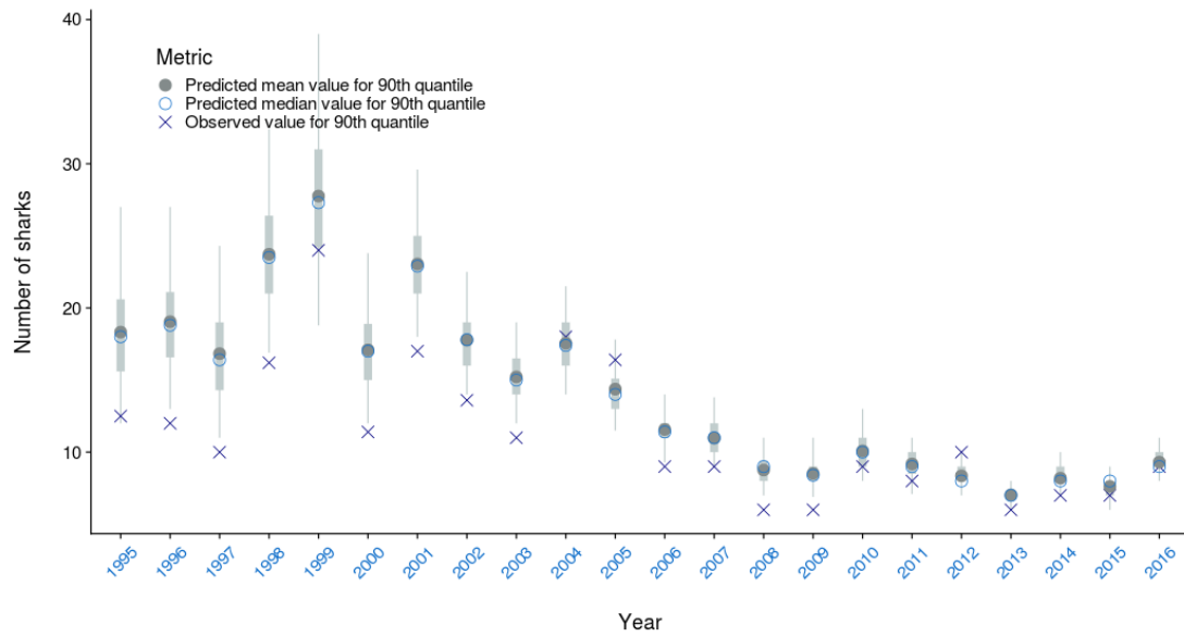
Figure A-30: Observed vs. predicted mean and median position of the 90 th quantile of oceanic whitetip shark caught by fishing event where catch > 0 by year for the longline bycatch fleet. The median \pm 25 th quantiles for the predictions is shown in grey; the whiskers cover the 2.5 - 97.5 th quantile range.
