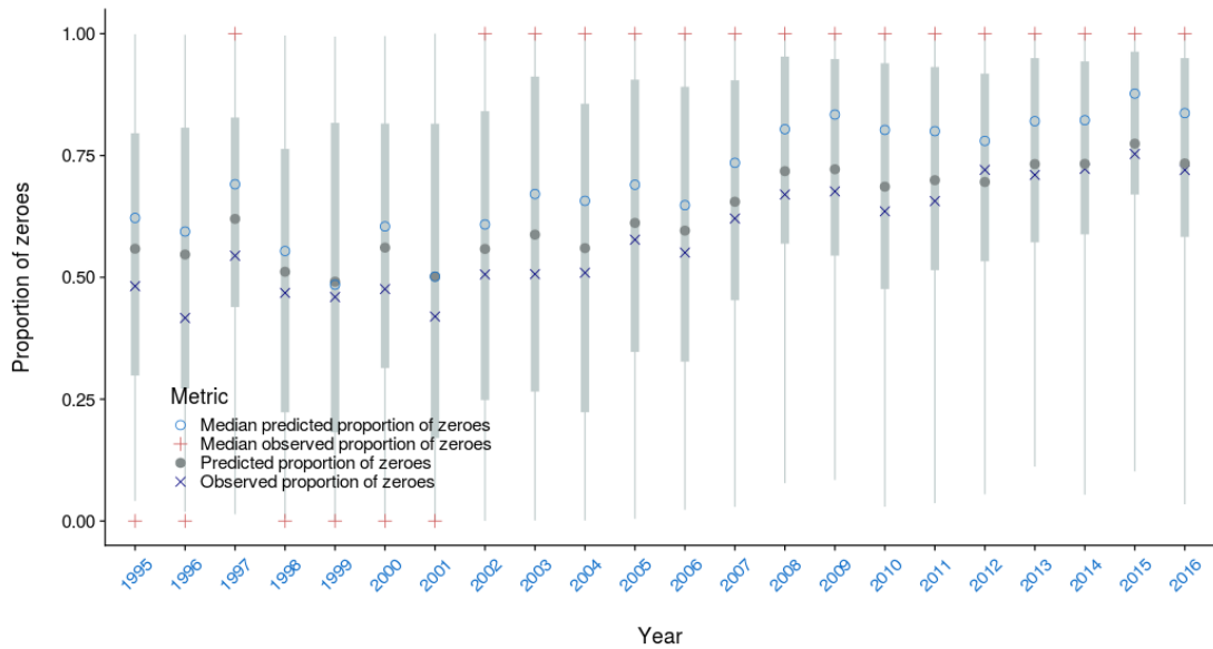
Figure A-24: Mean and median proportion of zero observed vs. predicted by fishing event for the observer catch rate model for the longline bycatch fleet by year. The median \pm 25 th quantiles for the predictions is shown in grey; the whiskers cover the 2.5-97.5 th quantile range.
