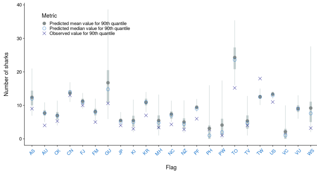
Figure A-31: Observed vs. predicted mean and median position of the 90 th quantile of oceanic whitetip shark caught by fishing event where catch > 0 by flag for the longline bycatch fleet. The median \pm 25 th quantiles for the predictions is shown in grey; the whiskers cover the 2.5 - 97.5 th quantile range.
