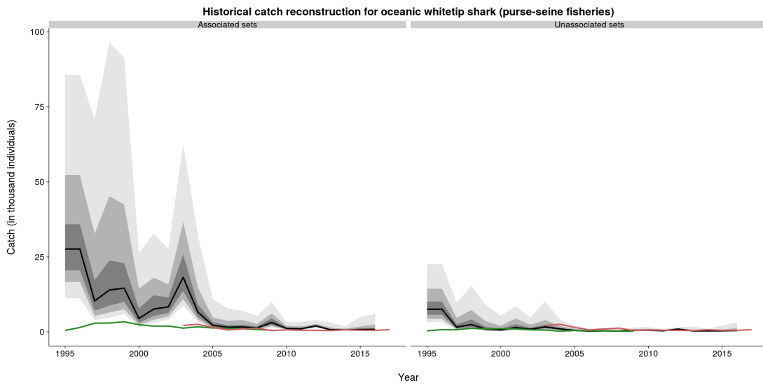
Figure 17: Median predictions of oceanic whitetip shark catch in the WCPO for the associated and unassociated purse-seine fleets based on a model of purse-seine observed catch rates applied to SBEST effort. The light, dark and darker grey bounds show the 0.025 th -0.975 th , 0.10 th -0.90 th and 0.25 th -0.75 th uncertainty bounds. For comparison with our estimates, the red line shows the prediction of historical catch published in (Peatman et al. 2018b) for these fleets and the green line shows the corresponding historical catches used in the reference case for the 2012 assessment.
