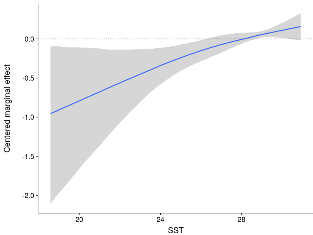
Figure 6: Predicted relationship between sea surface temperature (SST) and observed catch rates for the oceanic whitetip shark for the longline target fleet, independent of other covariates.
