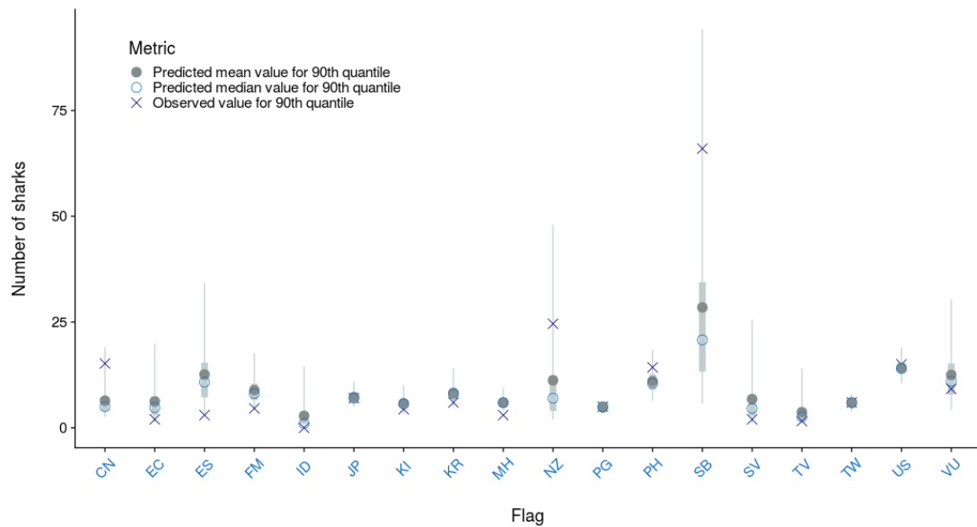
Figure A-51: Observed vs. predicted mean and median position of the 90 th quantile of oceanic whitetip shark caught by fishing event where catch > 0 by flag for the purse seine fleet. The median \pm 25 th quantiles for the predictions is shown in grey; the whiskers cover the 2.5 - 97.5 th quantile range.
