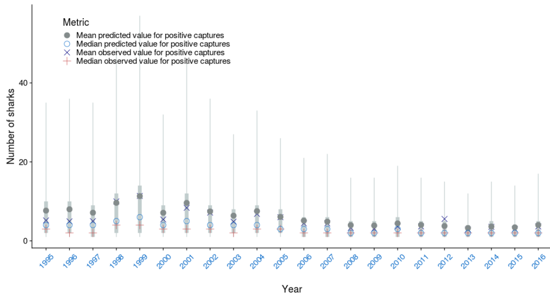
Figure A-27: Observed vs. predicted mean and median number of oceanic whitetip shark caught by fishing event where catch > 0 by year for the observer catch rate model for the longline bycatch fleet. The median \pm 25 th quantiles for the predictions is shown in grey; the whiskers cover the 2.5-97.5 th quantile range.
