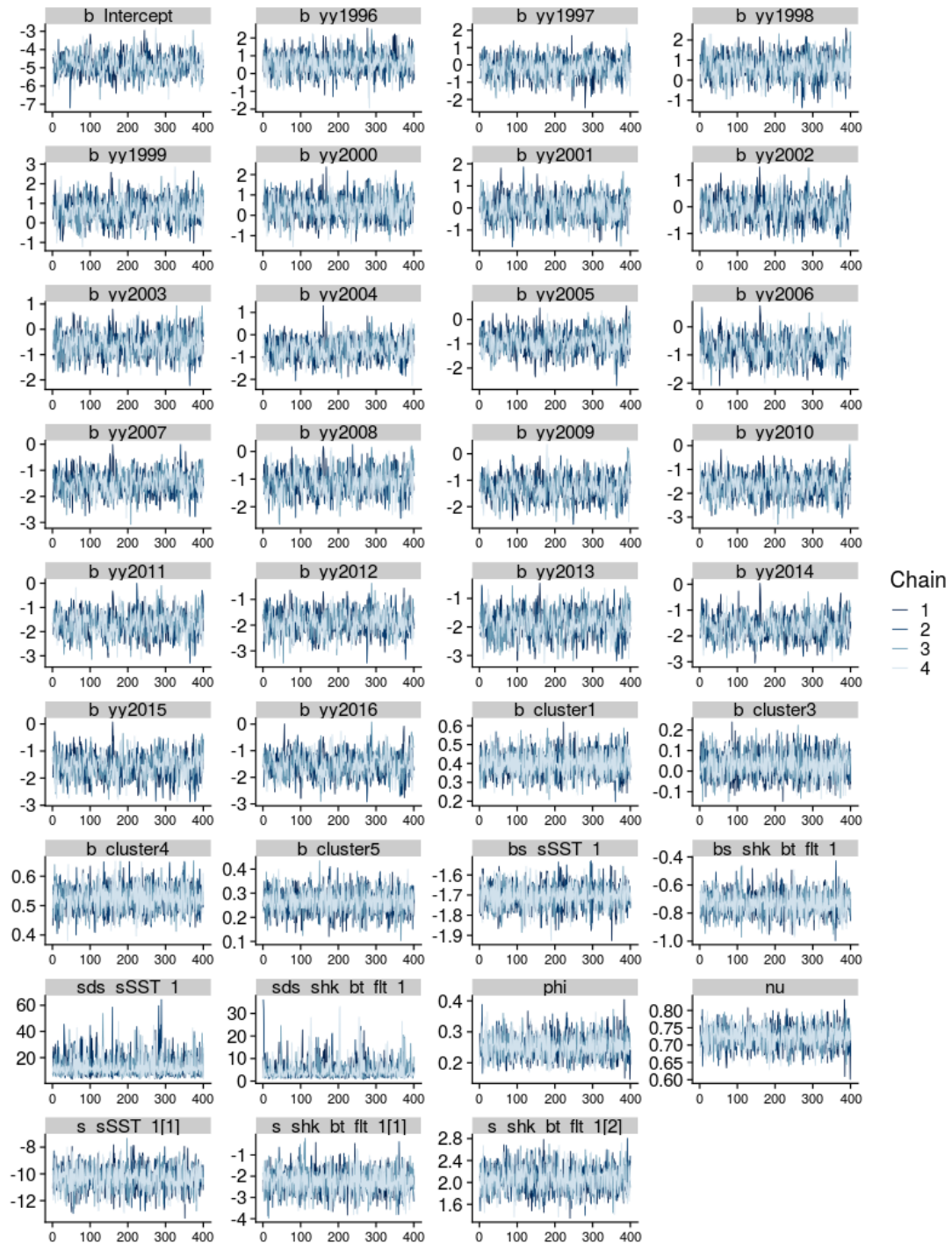
Figure A-63: Markov Chain Monte Carlo (MCMC) traces for key parameters of the observer catch rate model for the longline bycatch fleet. Chains (4) are shown in different colours.
