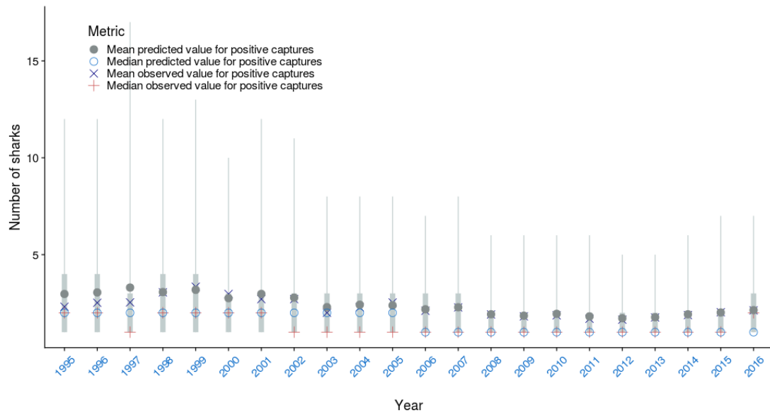
Figure A-57: Observed vs. predicted mean and median number of oceanic whitetip shark caught by fishing event where catch > 0 by year for the observer catch rate model for the longline bycatch fleet. The median \pm 25 th quantiles for the predictions is shown in grey; the whiskers cover the 2.5 - 97.5 th quantile range.
