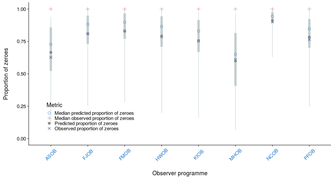
Figure A-55: Mean and median proportion of zero observed vs. predicted by fishing event for the observer catch rate model for the longline bycatch fleet by observer programme. The median \pm 25 th quantiles for the predictions is shown in grey; the whiskers cover the 2.5 - 97.5 th quantile range.
