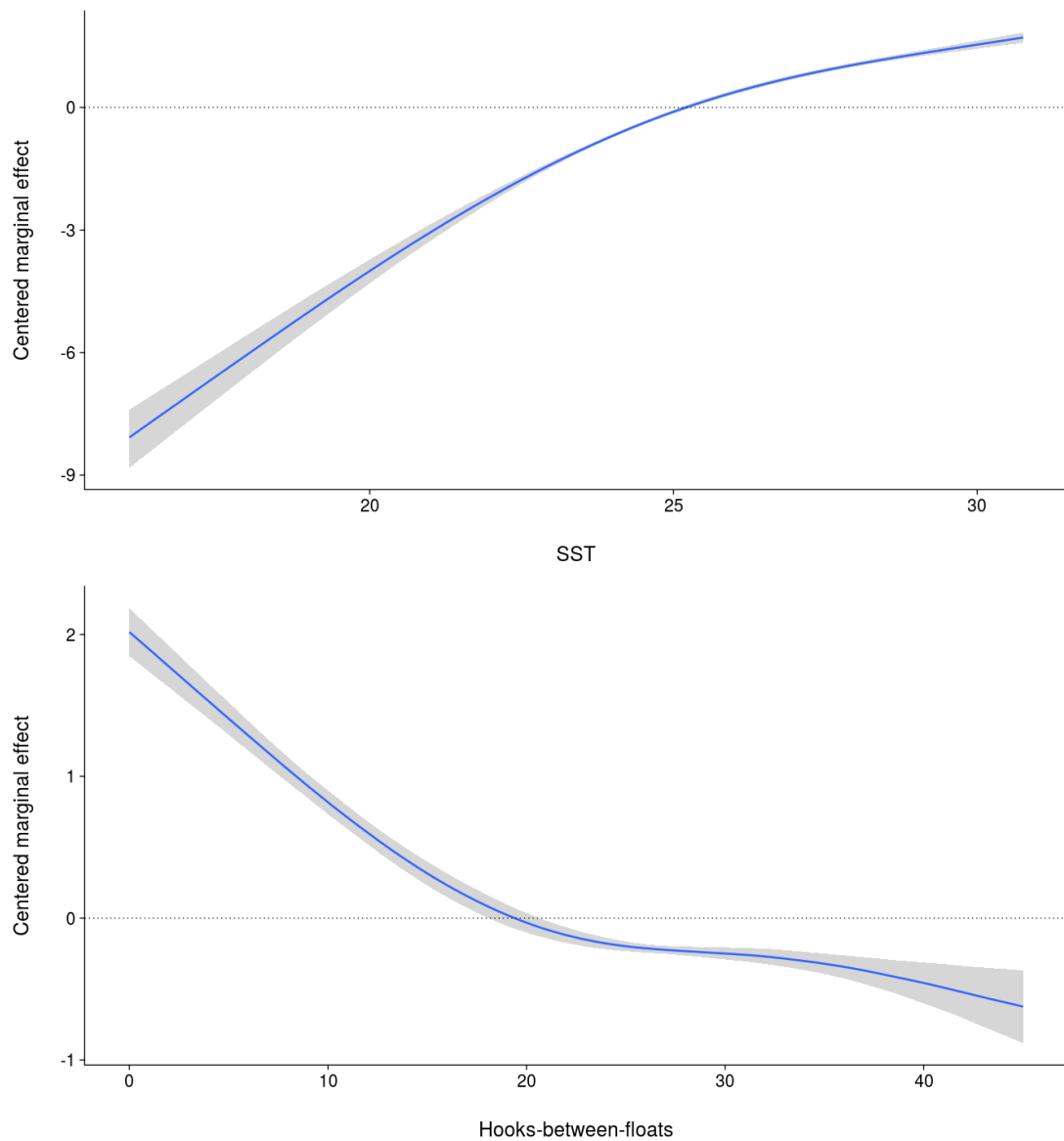
Figure 21: Predicted relationship for the observed catch rates for the oceanic whitetip shark vs. SST (top) and hooks - between - floats (bottom) in the model for the CPUE standardization based on the longline bycatch fleet, independent of other covariates.
