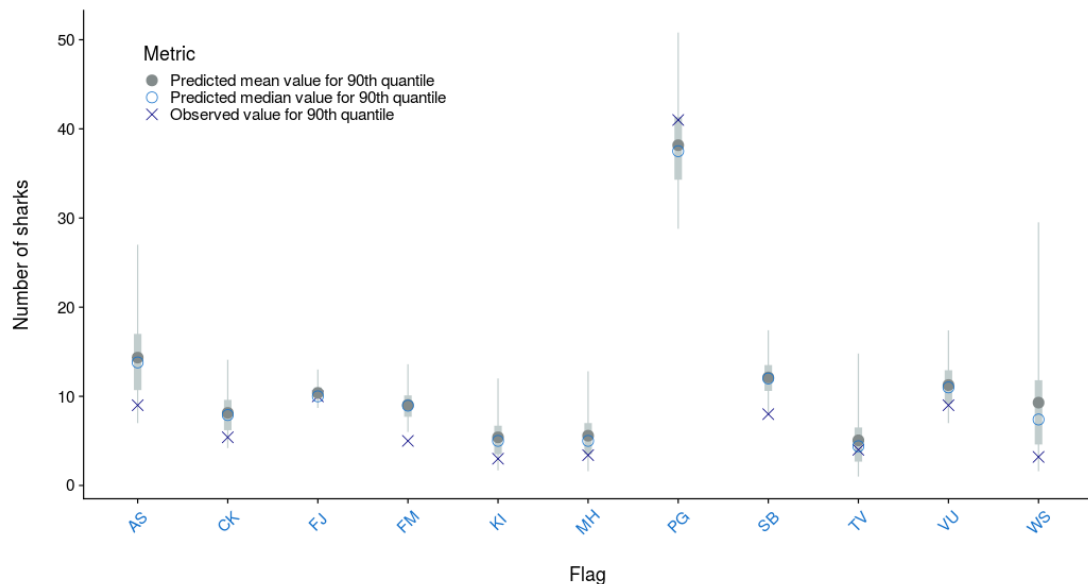
Figure A-41: Observed vs. predicted mean and median position of the 90 th quantile of oceanic whitetip shark caught by fishing event where catch > 0 by flag for the longline target fleet. The median ± 25 th quantiles for the predictions is shown in grey; the whiskers cover the 2.5 - 97.5 th quantile range.
