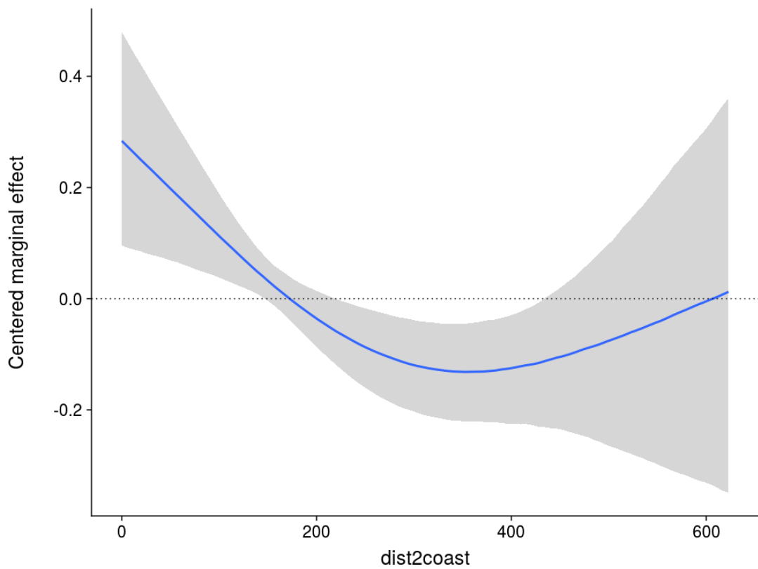
Figure 9: Predicted relationship between distance to the coastlines and observed catch rates for the oceanic whitetip shark in the model for purse seine fleets, independent of other covariates.
