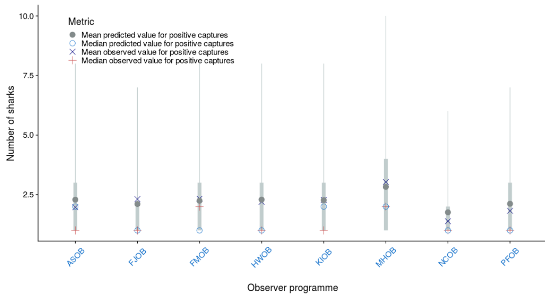
Figure A-58: Observed vs. predicted mean and median number of oceanic whitetip shark caught by fishing event where catch > 0 by observer programme for the observer catch rate model for the longline bycatch fleet. The median \pm 25 th quantiles for the predictions is shown in grey; the whiskers cover the 2.5 - 97.5 th quantile range.
