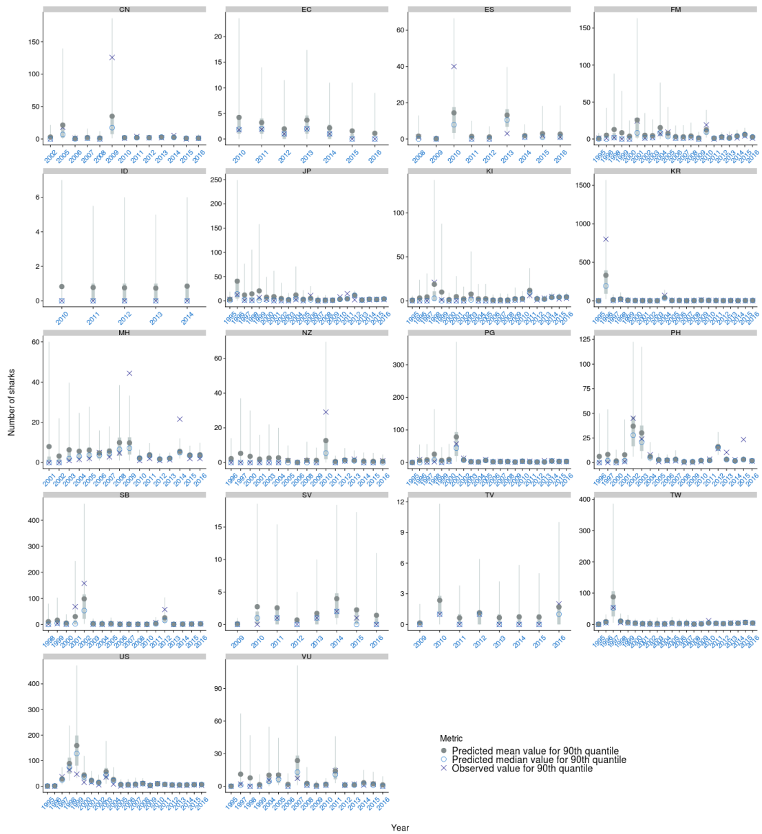
Figure A-52: Observed vs. predicted mean and median position of the 90 th quantile of oceanic whitetip shark caught by fishing event where catch > 0 by flag and year for the purse seine fleet. The median \pm 25 th quantiles for the predictions is shown in grey; the whiskers cover the 2.5-97.5 th quantile range.
