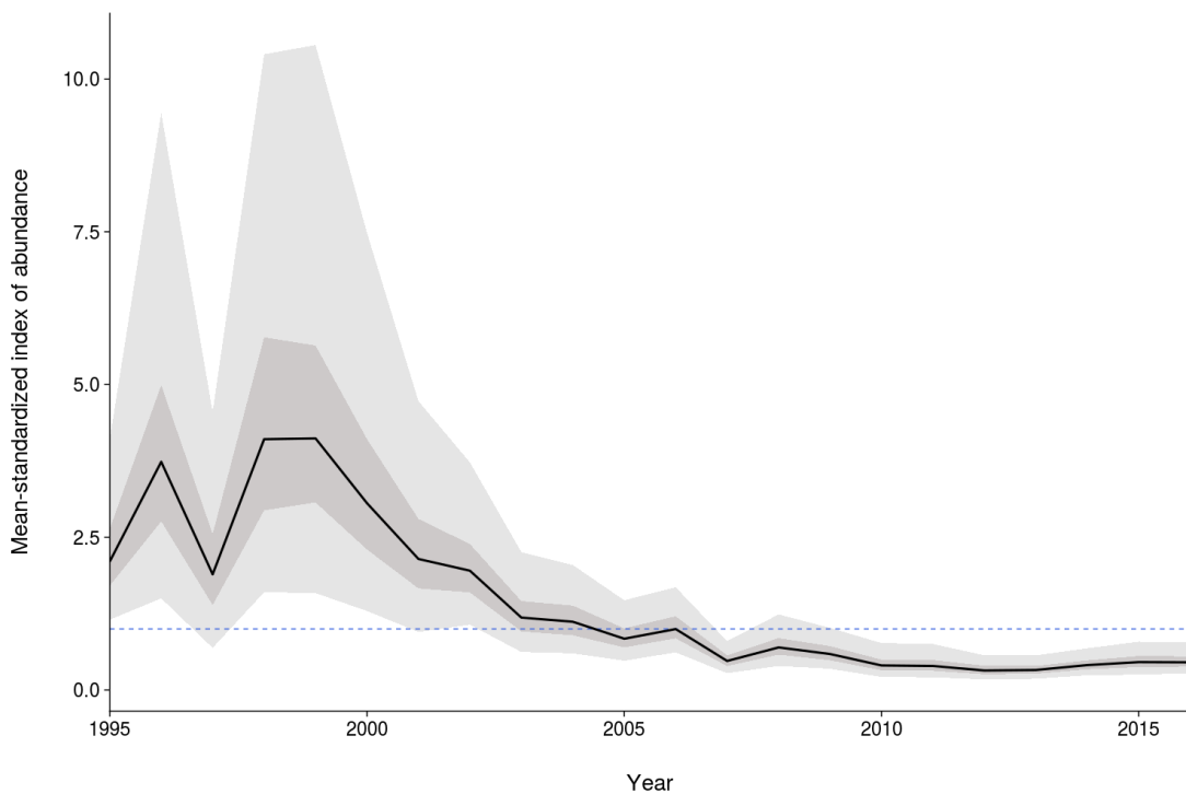
Figure 18: Mean-standardized CPUE index used in this assessment of oceanic whitetip shark. The light and dark grey bounds show the 0.025 th -0.975 th and 0.25 th -0.75 th uncertainty bounds around the year effects. The dashed line at 1 shows the reference mean value.
