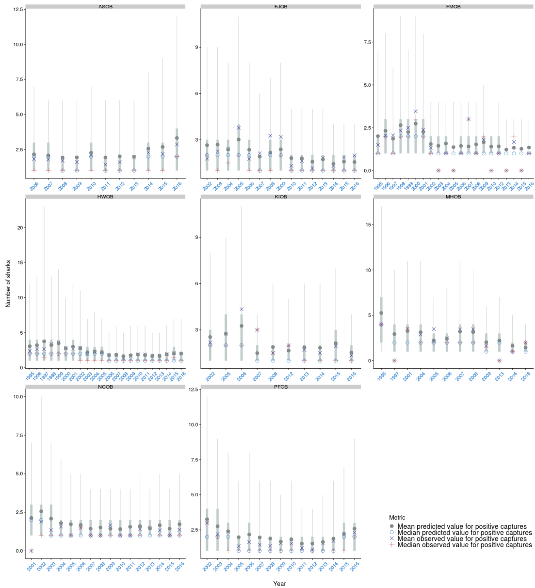
Figure A-59: Observed vs. predicted mean and median number of oceanic whitetip shark caught by fishing event where catch > 0 by observer programme and year for the observer catch rate model for the longline bycatch fleet. The median \pm 25 th quantiles for the predictions is shown in grey; the whiskers cover the 2.5-97.5 th quantile range.
