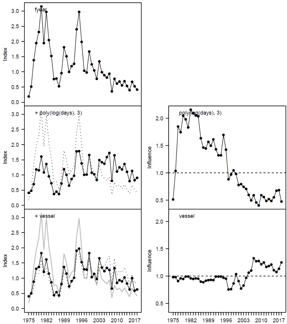
Figure A2: Step and influence plots for the East Northland charter vessel model.
