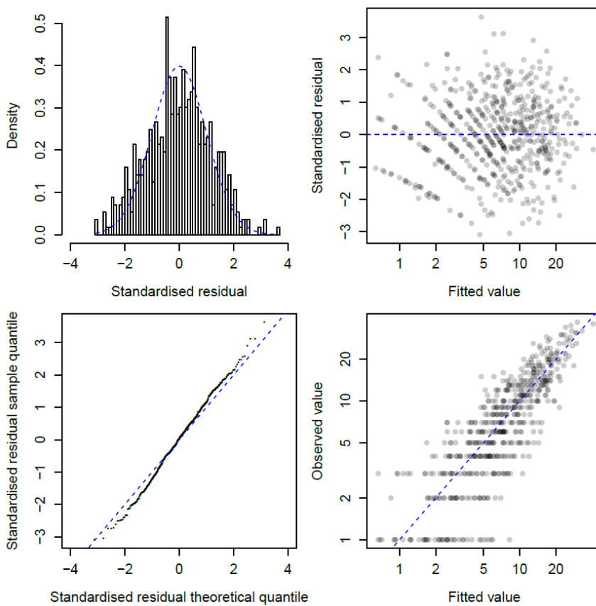
Figure 6: Residual diagnostics for the charter vessel model. Top left: histogram of standardised residuals compared to standard normal distribution.', Bottom left: quantile-quantile plot of standardised residuals.
