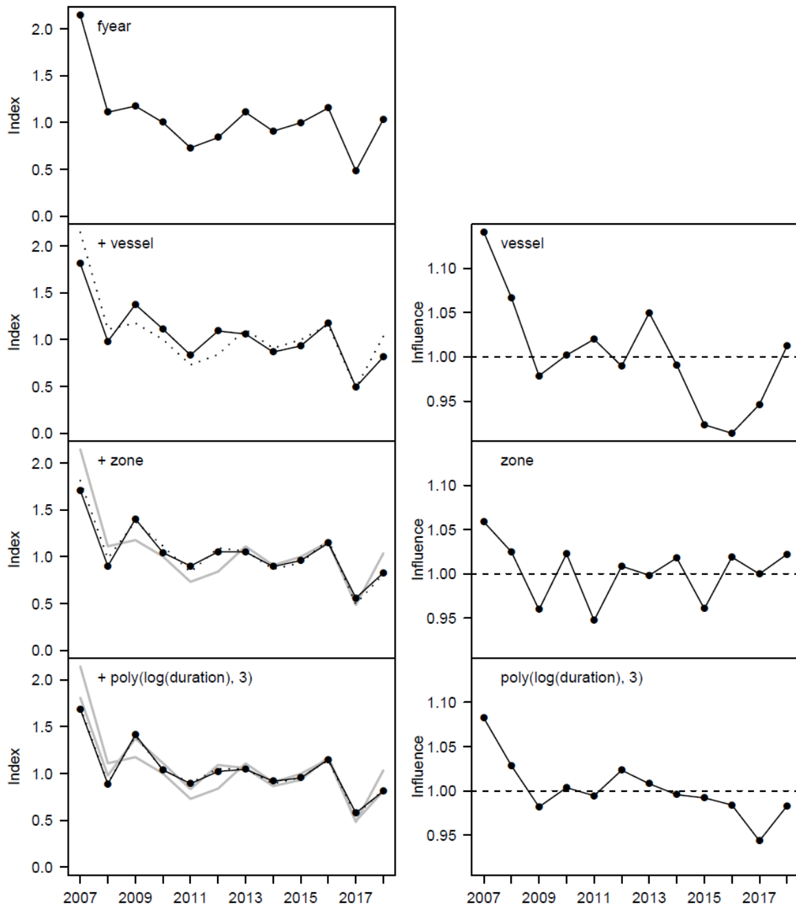
Figure B2: Step and influence plot from the billfish logbook model.
