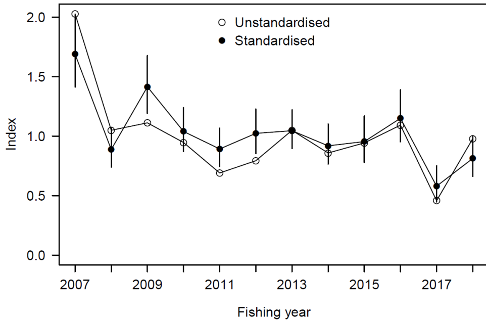
Figure 7: Overall standardization effect from the billfish logbook model of striped marlin CPUE. The unstandardised index is based on the geometric mean of the catch per year and is not adjusted for effort.
