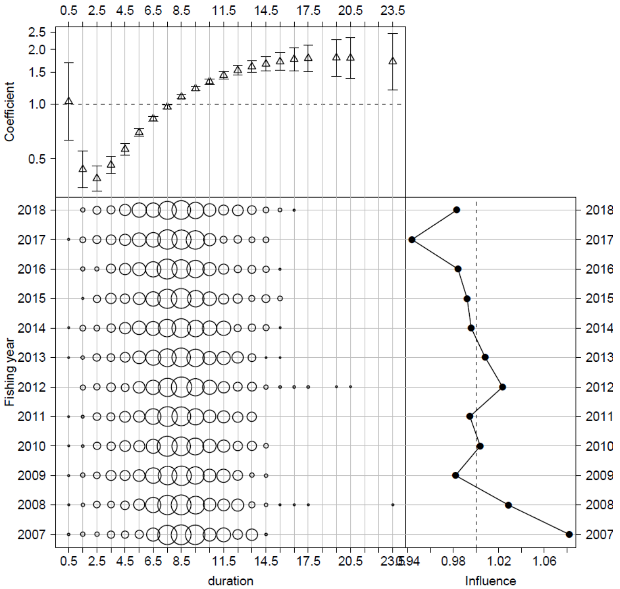
Figure B5: Coefficient-distribution-influence plot for poly(\log(\text{duration}), 3) from the billfish logbook model.
