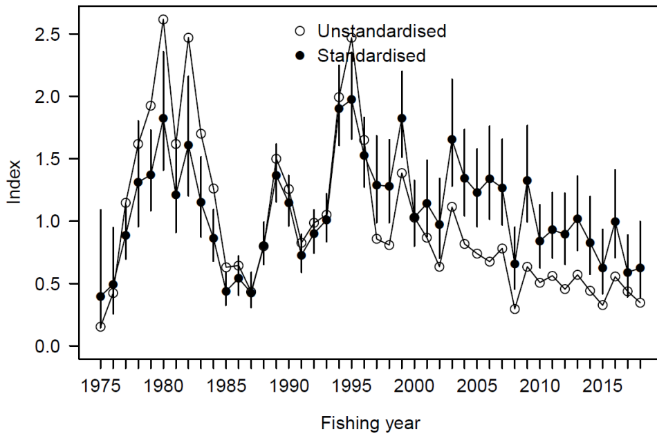
Figure 5: Overall standardization effect of the East Northland charter vessel model of striped marlin CPUE. The unstandardized index is based on the geometric mean of the catch per year and is not adjusted for effort.
