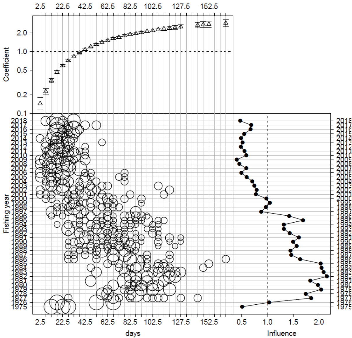
Figure A3: Coefficient-distribution-influence plot for poly(\log(days), 3) for the East Northland charter vessel model.
