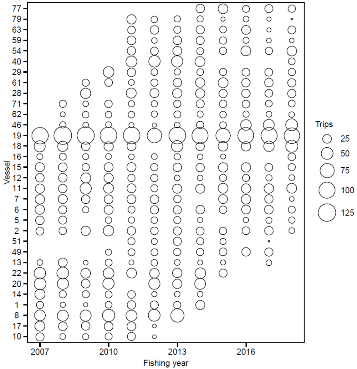
Figure B1: Number of trips by fishing year for core vessels providing billfish logbook data. The area of circles is proportional to the number of trips for a vessel in a fishing year.
