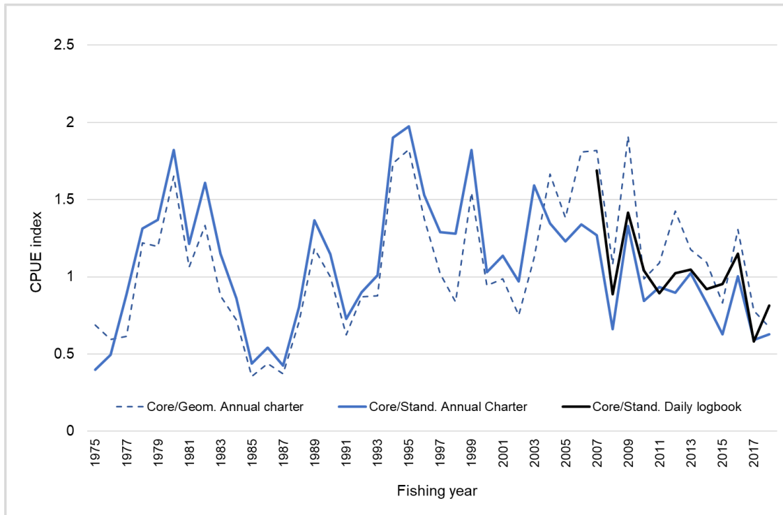
Figure 9: Comparison between the negative binomial model of East Northland recreational charter boat annual CPUE since 1975 and billfish logbook daily CPUE since 2007.
