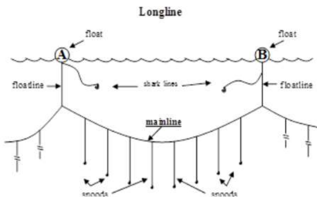
Annex 1: Schematic diagram of a shark line
