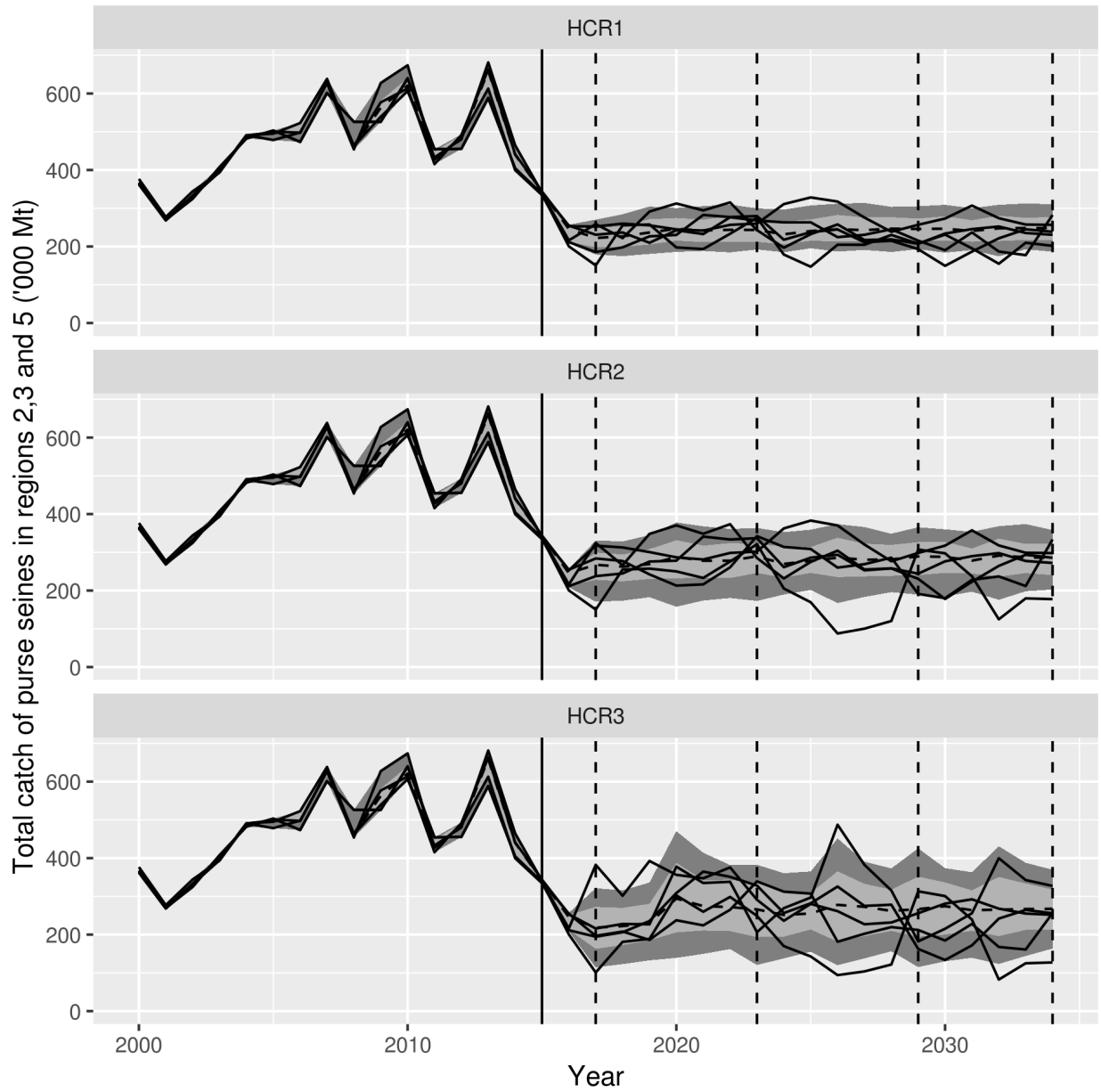
Figure 21: Expected catch of the purse seine fisheries in regions 2,3, and 5 for the three HCRs. The ribbons show the 0.05-0.95 (dark grey) and 0.20-0.80 (light grey) percentiles. The dashed line is the median. The solid lines are example trajectories of 5 randomly selected simulations. The dashed vertical lines indicate the short-, medium- and long-term time periods over which the indicators are calculated.
