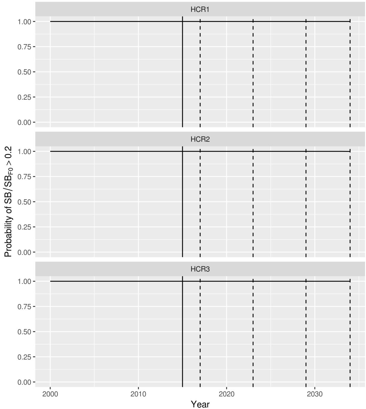
Figure 18: Probability of SB/SB_{F=0} > 0.2 for the whole region for the three HCRs. The solid vertical line at 2015 indicates the start of the projection. The dashed vertical lines indicate the short-, medium- and long-term time periods over which the indicators are calculated.
