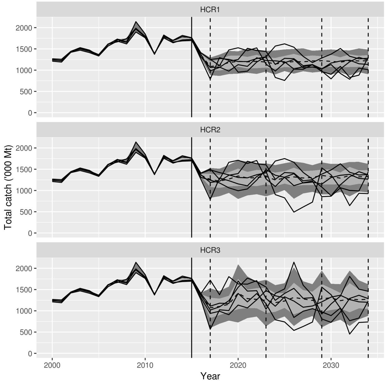
Figure 20: Expected total catch for the three HCRs. The ribbons show the 0.05-0.95 (dark grey) and 0.20-0.80 (light grey) percentiles. The dashed line is the median. The solid lines are example trajectories of 5 randomly selected simulations. The dashed vertical lines indicate the short-, medium- and long-term time periods over which the indicators are calculated.
