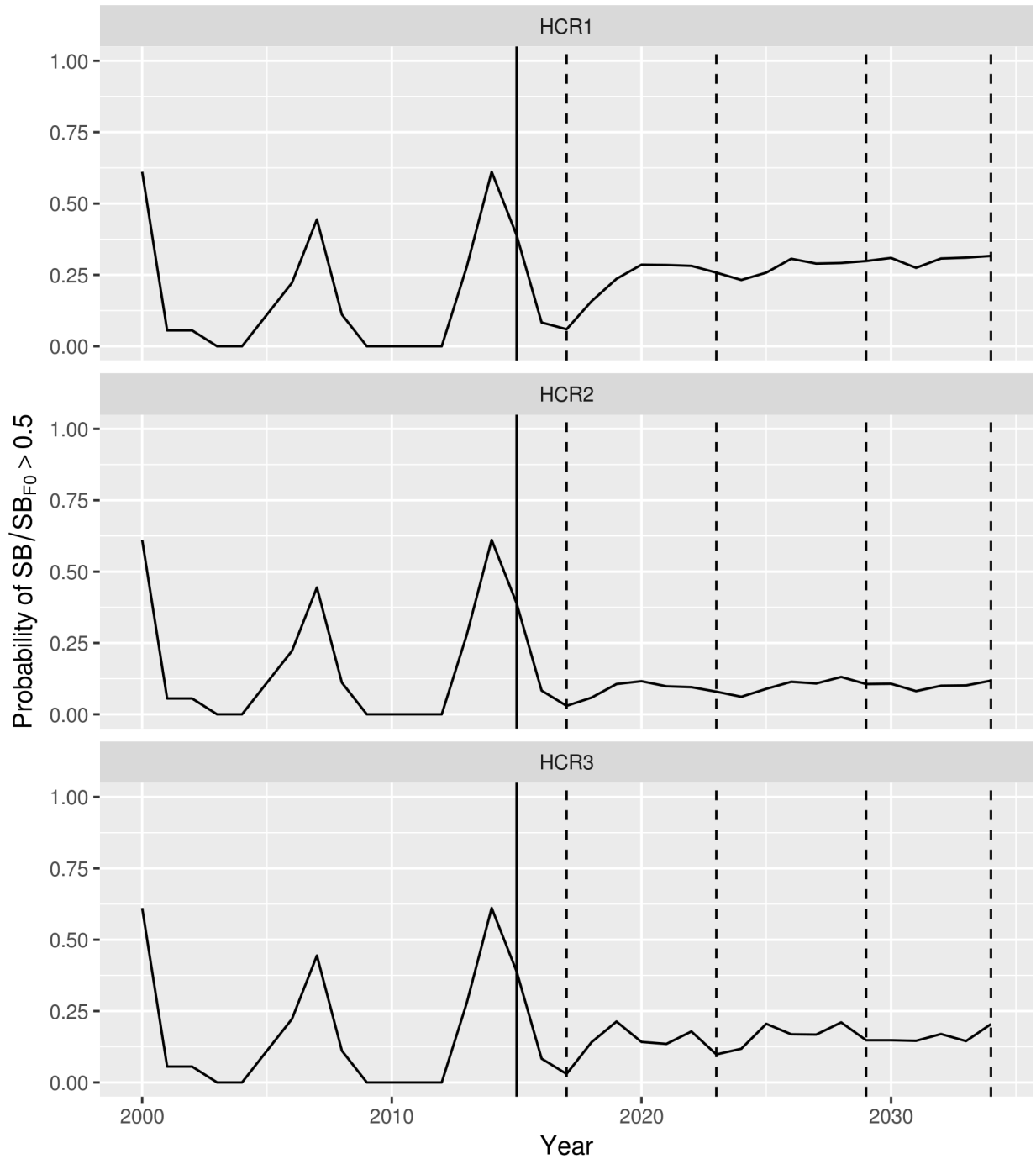
Figure 23: Probability of SB/SB_{F=0} > 0.5 for the whole region for the three HCRs. The solid vertical line at 2015 indicates the start of the projection. The dashed vertical lines indicate the short-, medium- and long-term time periods over which the indicators are calculated.
