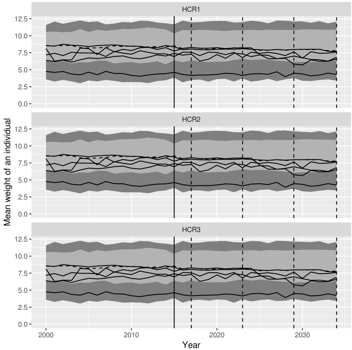
Figure 24: Mean weight of an individual across the total stock for the three HCRs. The ribbons show the 0.05-0.95 (dark grey) and 0.20-0.80 (light grey) percentiles. The dashed line is the median. The solid lines are example trajectories of 5 randomly selected simulations. The dashed vertical lines indicate the short-, medium- and long-term time periods over which the indicators are calculated.
