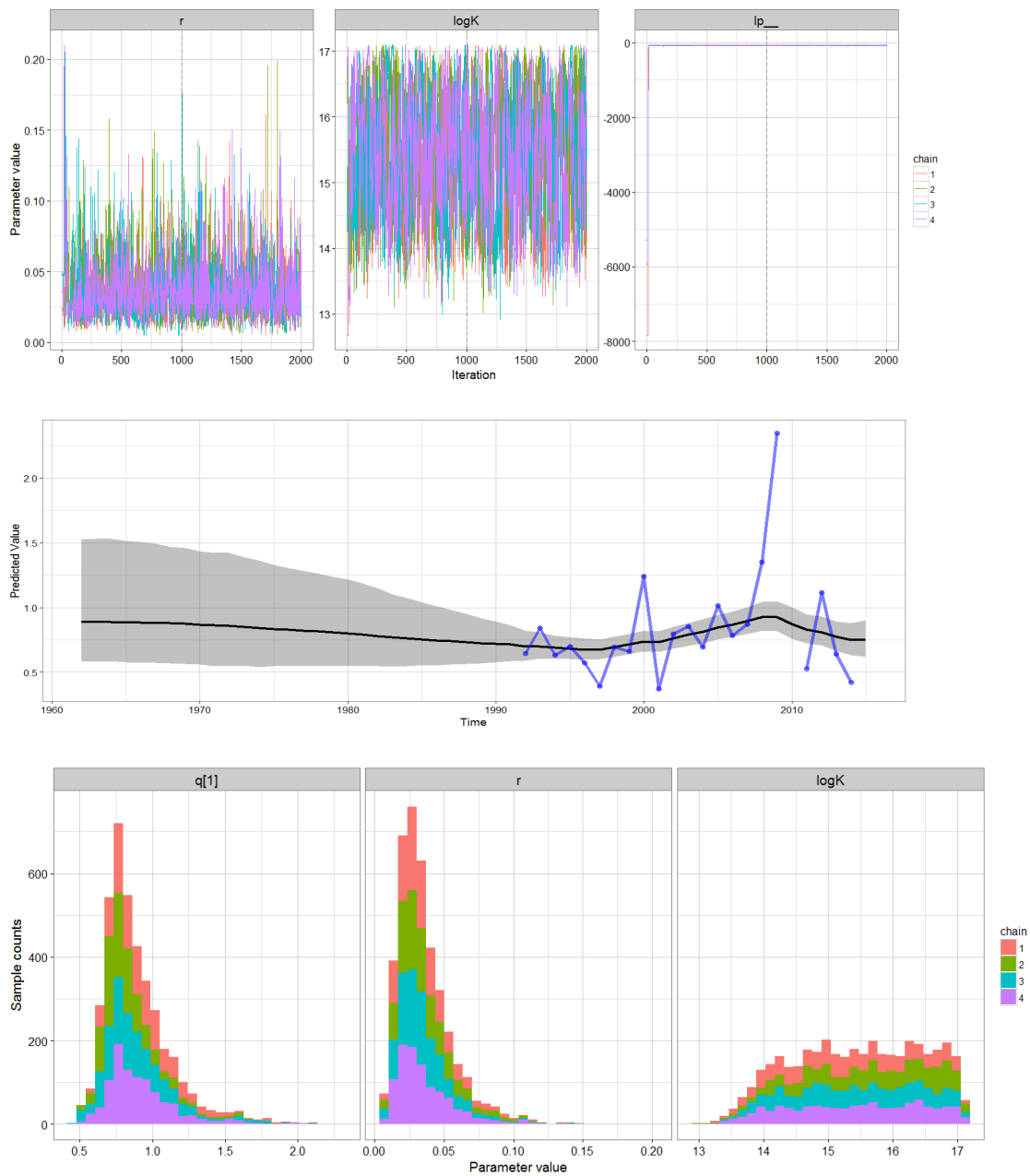
Figure 20. Top: Trace outputs from the MCMC model fit showing estimates of r and \log(K) alongside the log-posterior ( \log p_{\text{post}} ). Middle: Derived fit to the CPUE index. Bottom: Stacked histograms of MCMC samples, representing the posterior distributions of q , r and \log(K) .
