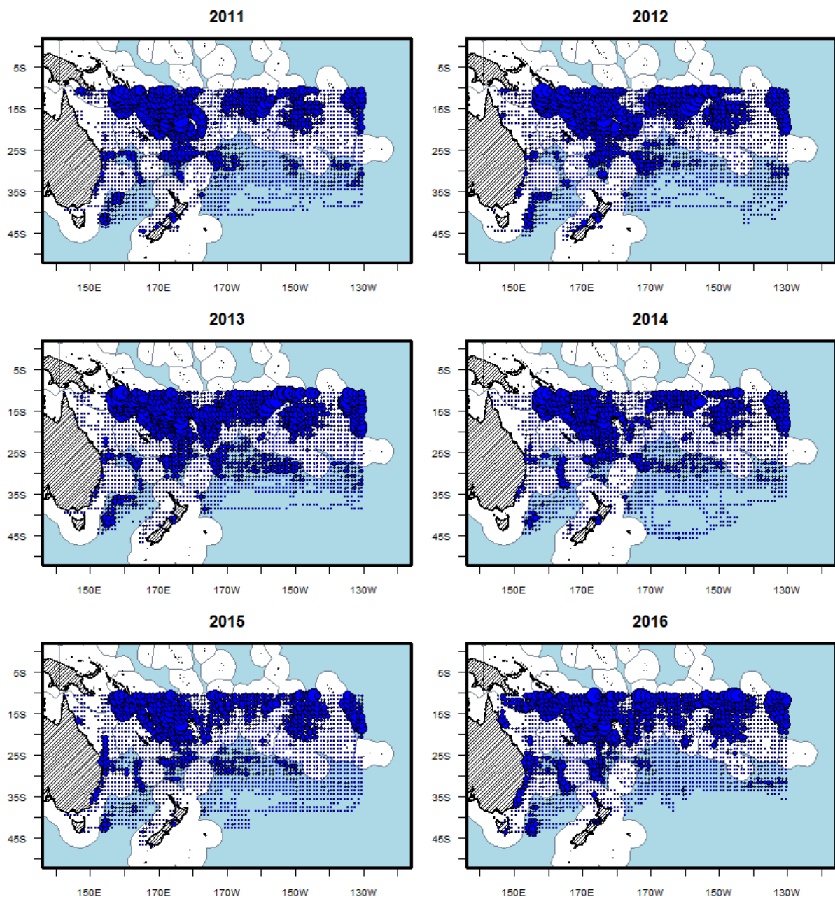
Figure 4: Longline VMS days-at-sea (augmented by logsheets) within the southern WCP-CA at 1^{\circ} \times 1^{\circ} (excluding archipelagic waters), south of 10^{\circ}S . Maximum circle size = 965 days.
