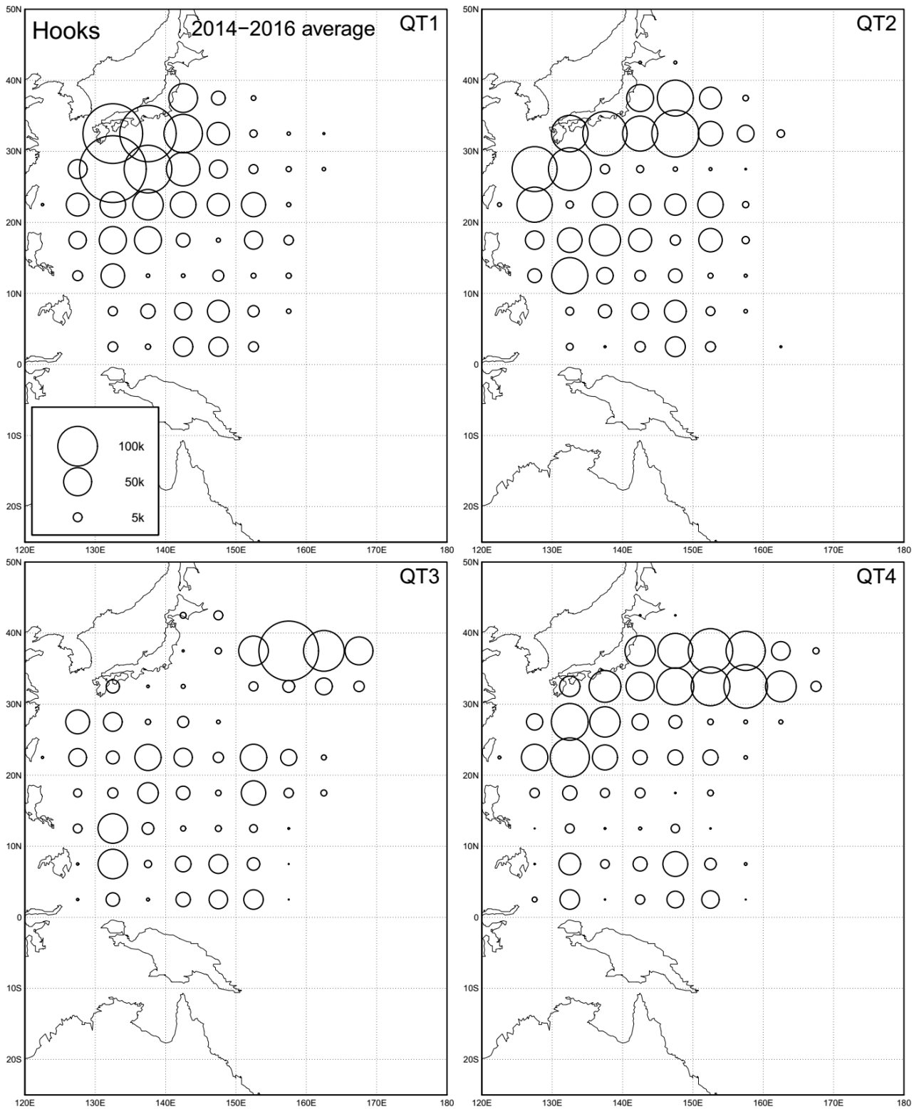
Fig. 5. Quarterly distribution of fishing effort for the Japanese small offshore longline fisheries (10- 20 GRT) in the western and central Pacific Ocean in average of 2014-2016.
