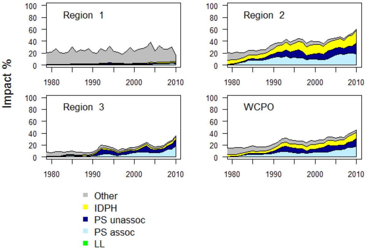
Figure SKJ4: Estimates of reduction in spawning potential due to fishing (fishery impact = 1 - SB_t / SB_{t_{R=0}} ) by region and for the WCPO attributed to various fishery groups (reference case model). L = all longline fisheries; IDPH = Philippines and Indonesian domestic fisheries; PS assoc = purse-seine log and FAD sets; PS unassoc = purse-seine school sets; Other = pole-and-line fisheries and coastal Japan purse-seine.
