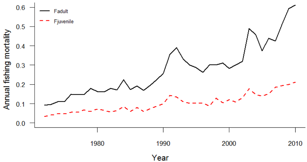
Figure SKJ3: Estimated annual average juvenile and adult fishing mortality for the WCPO obtained from the reference case model.
