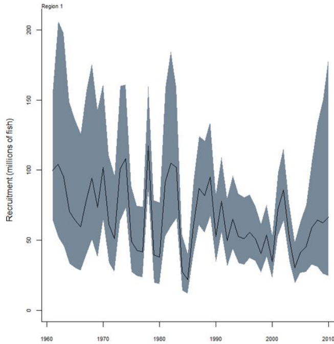
Figure ALB1: Annual recruitment (number of fish) estimates. The grey area represents parameter uncertainty estimated from the Hessian matrix.
