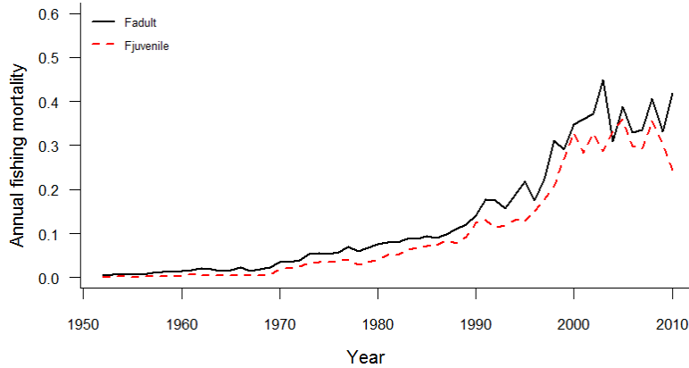
Figure YFT3: Estimated annual average juvenile and adult fishing mortality for the WCPO obtained from the base case model (LLcpueOP_TWcpueR6_PTTTP – H80pttp).
