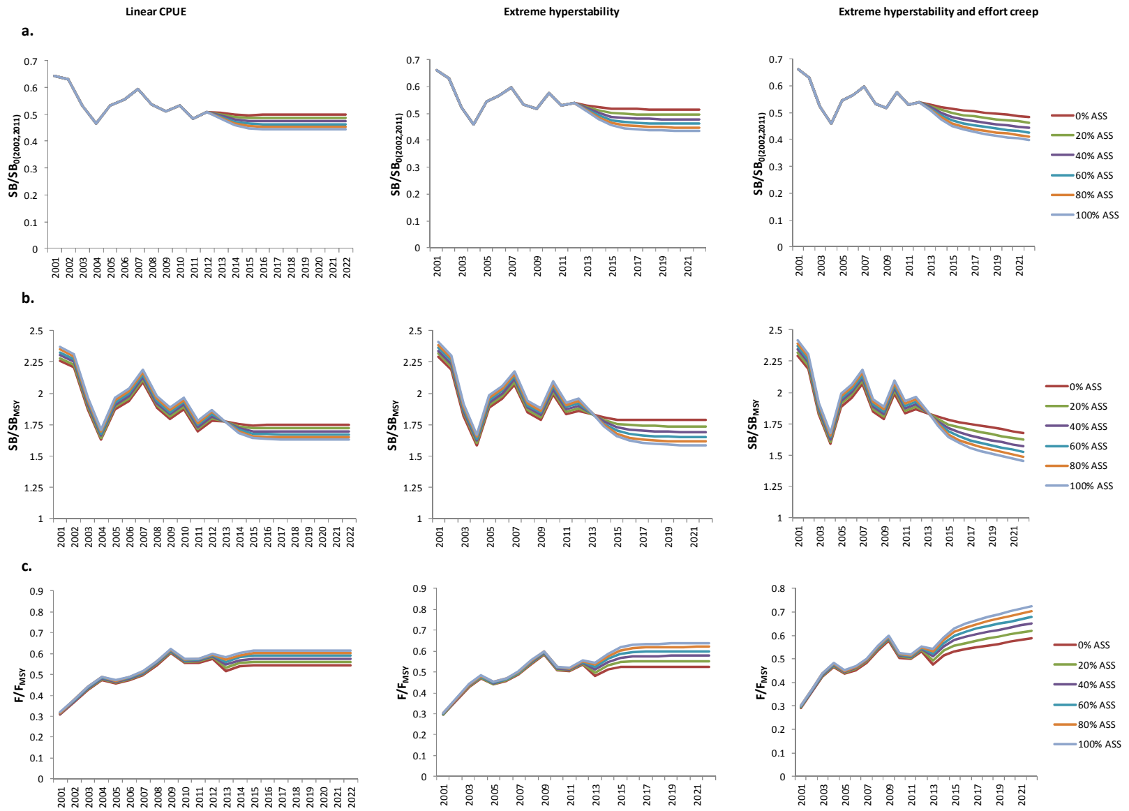
Figure 3. Projections of a) SB/SB_0(2002-2011) ; b) SB/SB_{MSY} ; and c) F/F_{MSY} with different proportions of total purse seine effort on associated (ASS) sets.
