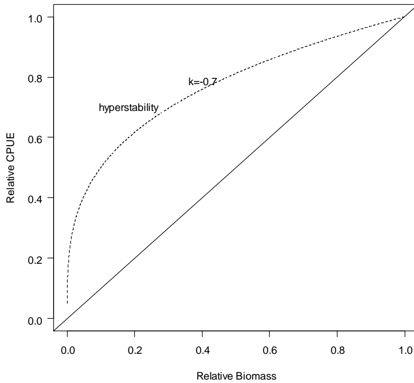
Figure 2. Conceptual plot of the assumed relationship between CPUE and stock abundance, for the two scenarios examined in this paper. Under extreme hyperstability ( K=-0.7 ), CPUE remains at high levels with decreasing abundance, resulting in hyperstability in CPUE.
