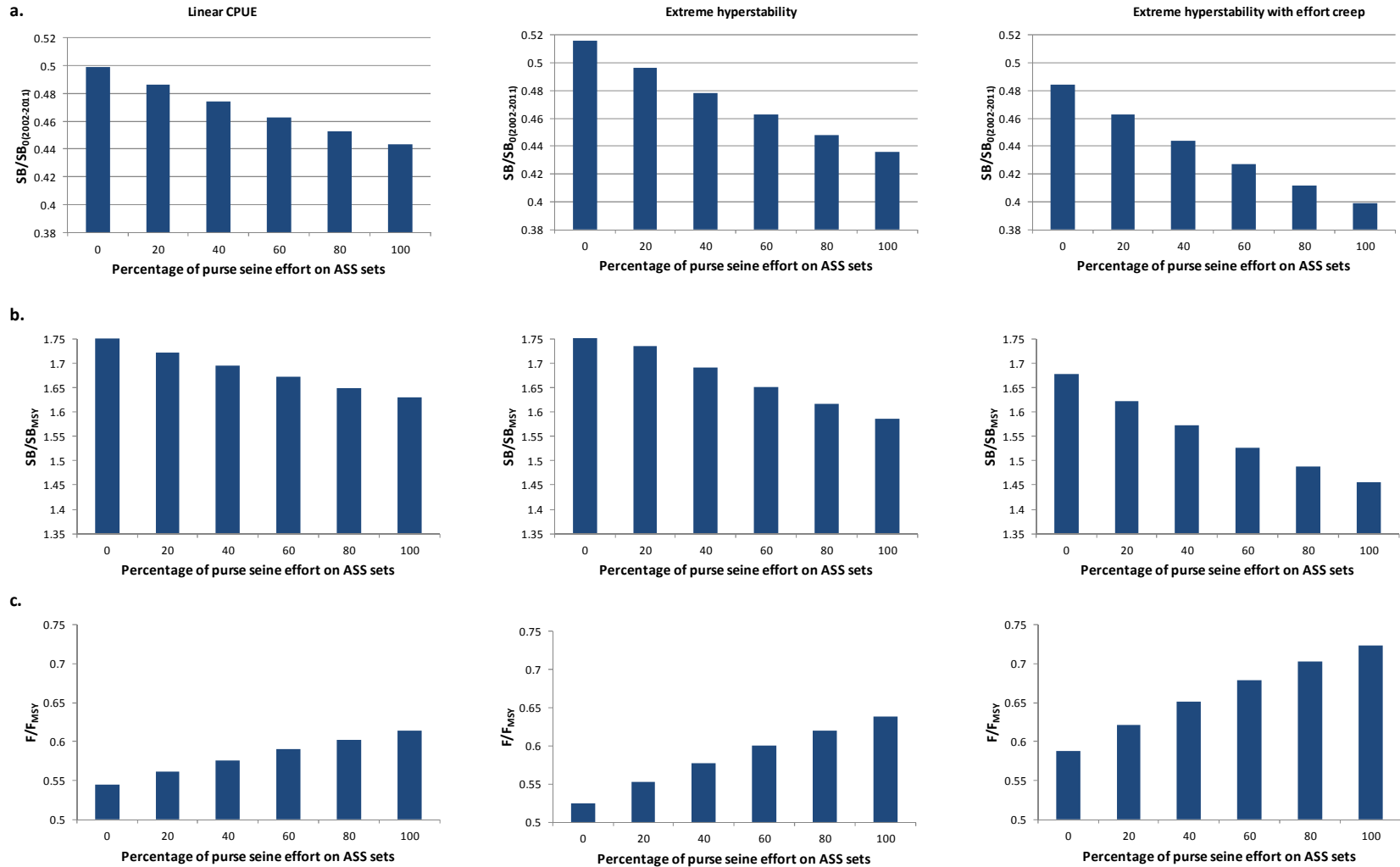
Figure 4. Response of stock status indicators a) SB_{2022}/SB_{F=0} (2002-2011); b) SB_{2022}/SB_{MSY} ; and c) F_{2022}/F_{MSY} to different proportions of total purse seine effort on associated (ASS) sets. NOTE: y-axis scales do not start at zero and hence differences are exaggerated.
