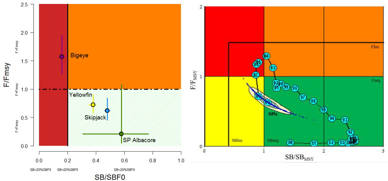
Figure 1. (a, left): "Majuro plot", with a coloring scheme that depicts stock status as Red at the biomass LRP (from WCPFC, 2014). (b, right): Traditional "Kobe Plot" with LRP indicated by additional horizontal and vertical lines (from IOTC, 2014).
