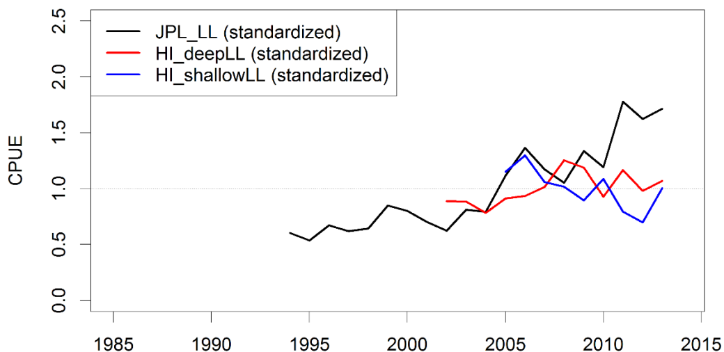
Figure E1. Standardized indices of abundance by fishery for shortfin mako sharks. While all of the available independent information was examined to draw conclusions about the stock, these three indices were considered to have the greatest value in determining stock status.
