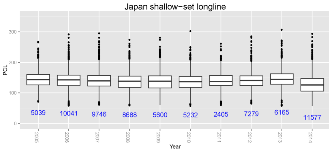
Figure 4.4. Boxplots (showing medians, interquartile ranges, 1.5 times the interquartile ranges, and outliers) of the annual sizes of shortfin mako sharks caught in North Pacific surveys and fisheries.
