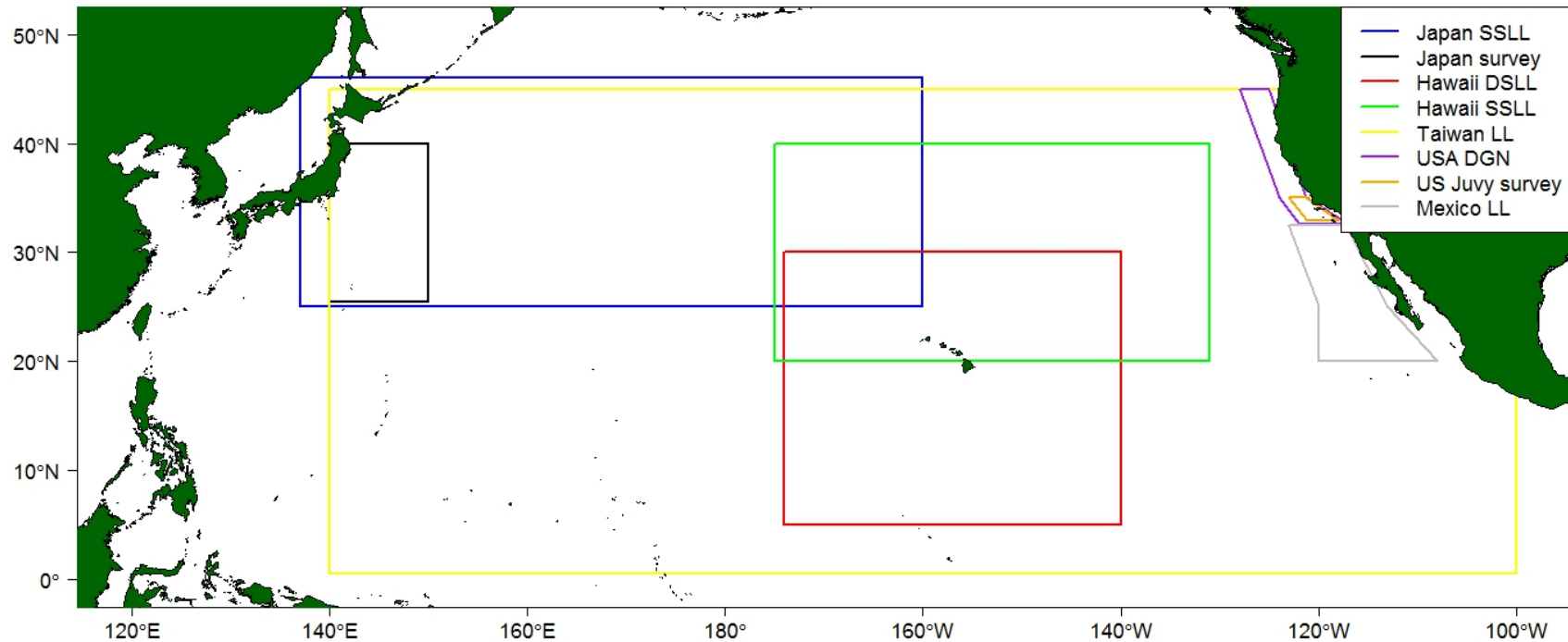
Figure 3.3. Spatial extent of the fisheries for which CPUE time series were developed. Fisheries include Japan shallow-set longline (Japan SSSL), Japan longline survey (Japan survey), Hawaii-based deep-set longline (Hawaii DSLL), Hawaii-based shallow-set longline (Hawaii SSLL), Taiwan distant water longline (Taiwan LL), U.S. west coast large-mesh drift gillnet (USA DGN), U.S. juvenile shark longline survey (US Juvy survey), and Mexico longline (Mexico LL).
