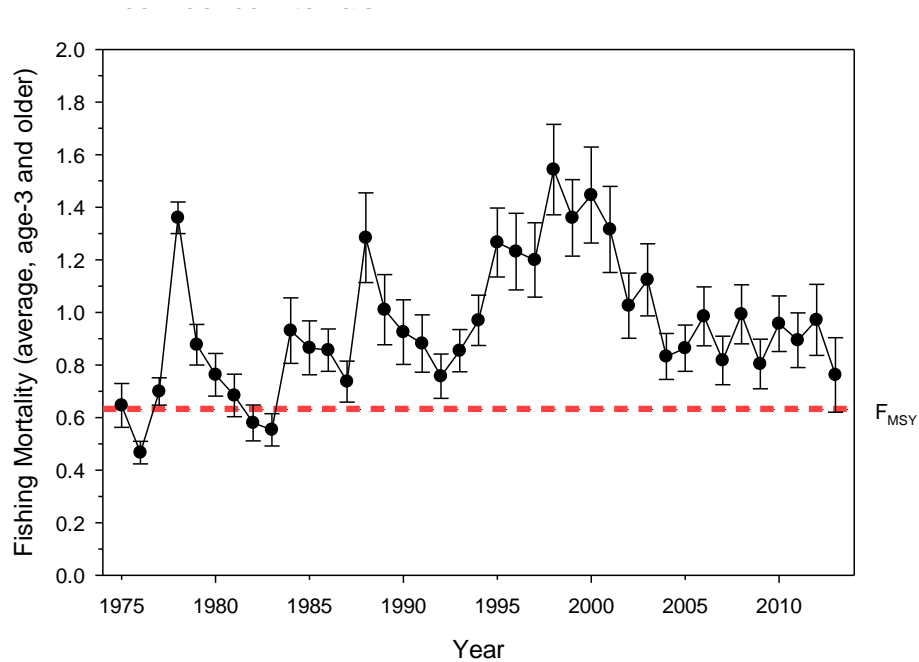
Figure C. Trends in estimates of fishing mortality of Western and Central North Pacific striped marlin ( Kajikia audax ) during 1975-2013 along with 80% confidence intervals.
