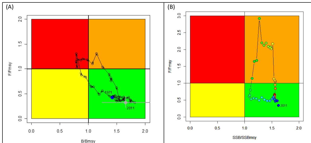
Figure 7-15. (A) Kobe plot showing median biomass and fishing mortality trajectories for the reference case Bayesian Surplus Production model for North Pacific blue shark ( Prionace glauca ). Solid blue circle indicates the median estimate in 1971 (initial year of the model). Solid gray circle and its horizontal and vertical bars indicate the median and 90% confidence limits in 2011. Open black circles and black arrows indicate the historical trajectory of stock status between 1971 and 2011. (B) Kobe plot showing estimated spawning biomass and fishing mortality trajectories for the reference case Stock Synthesis model for North Pacific blue shark. The circles indicate the historical trajectory from 1971-2011 colored from red (first year) to blue (terminal year).
