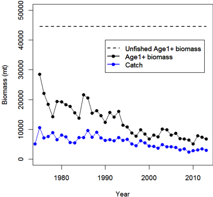
Figure 7-6. Trend in population biomass and reported catch biomass of Western and Central North Pacific striped marlin ( Kajikia audax ) during 1975-2013 relative to unfished biomass.
