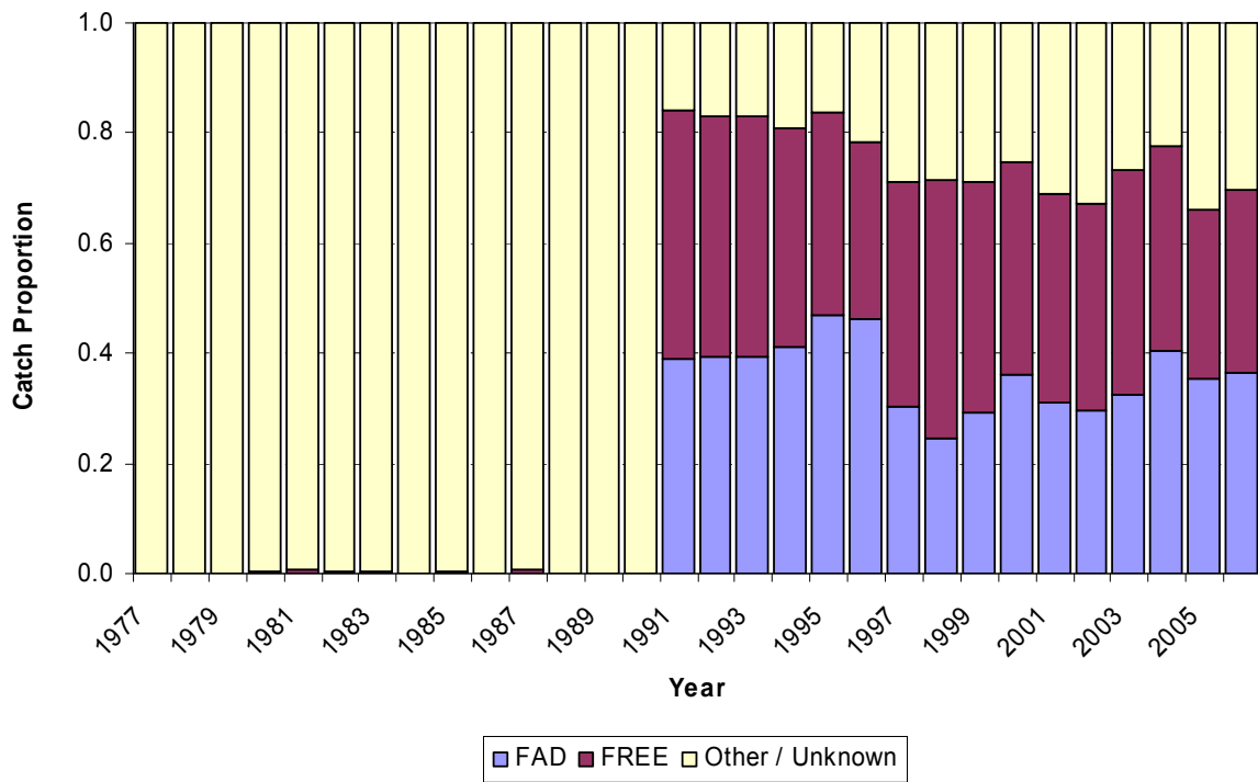
Figure 7 Purse Seine Catch Proportion (FAD vs Free) Atlantic Ocean 1977-2006
