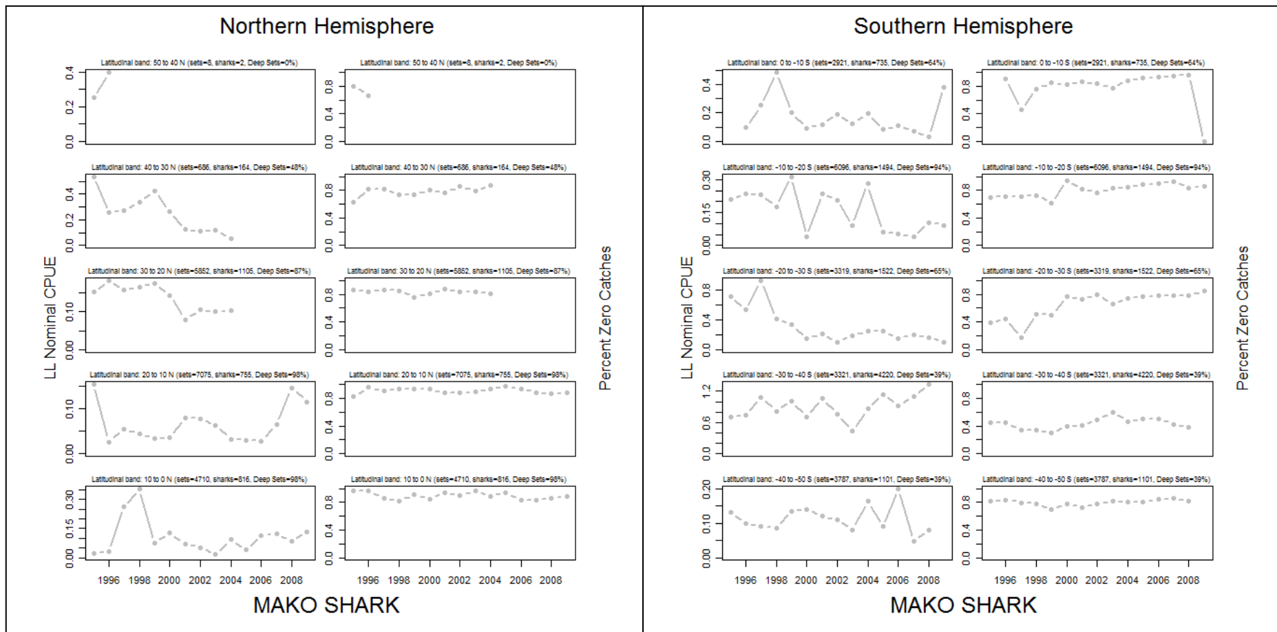
Figure A4 (cont.) Paired plots of nominal catch rates (left) and proportion of sets with zero catch (right) for mako sharks in 10^{\circ} latitudinal bands for the northern and southern hemispheres. Each panel shows the number of sets represented, the number of sharks represented and the percentage of sets that were fished deep (i.e. with \geq 10 hooks per basket).
