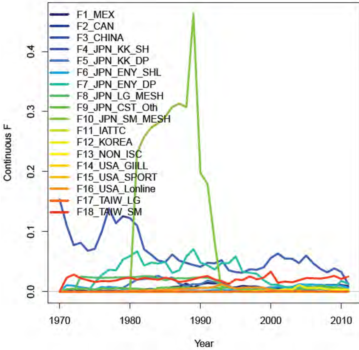
Figure 31. Estimated fishing mortality for each fishing gear for the SS reference case model.
