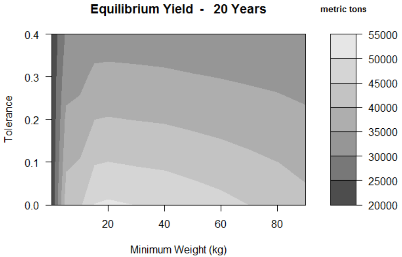
Figure 9. Isopleths of equilibrium yield given expanded minimum weight range to explore the YPR relationship. Note the rapid rise in yield that starts at approximately a 10 kg minimum weight and reaches a maximum around 20 kg.
