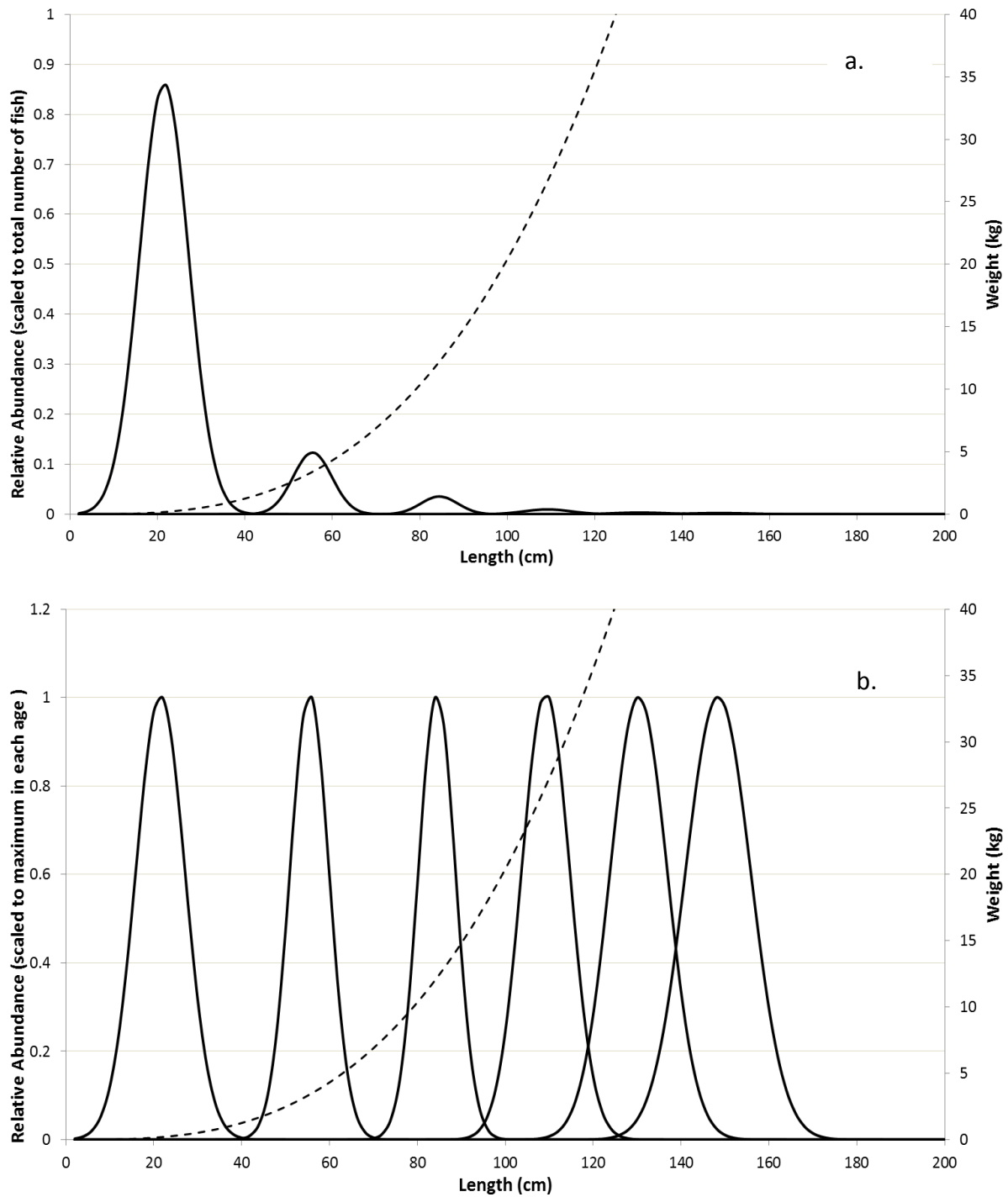
Figure 1. The relative abundance of ages 0 – 5 as scaled to the total abundance is presented in 1a. Figure 1b has normalized each cohort to the maximum number in each age. On both plates, the corresponding length weight relationship has been overlaid.
