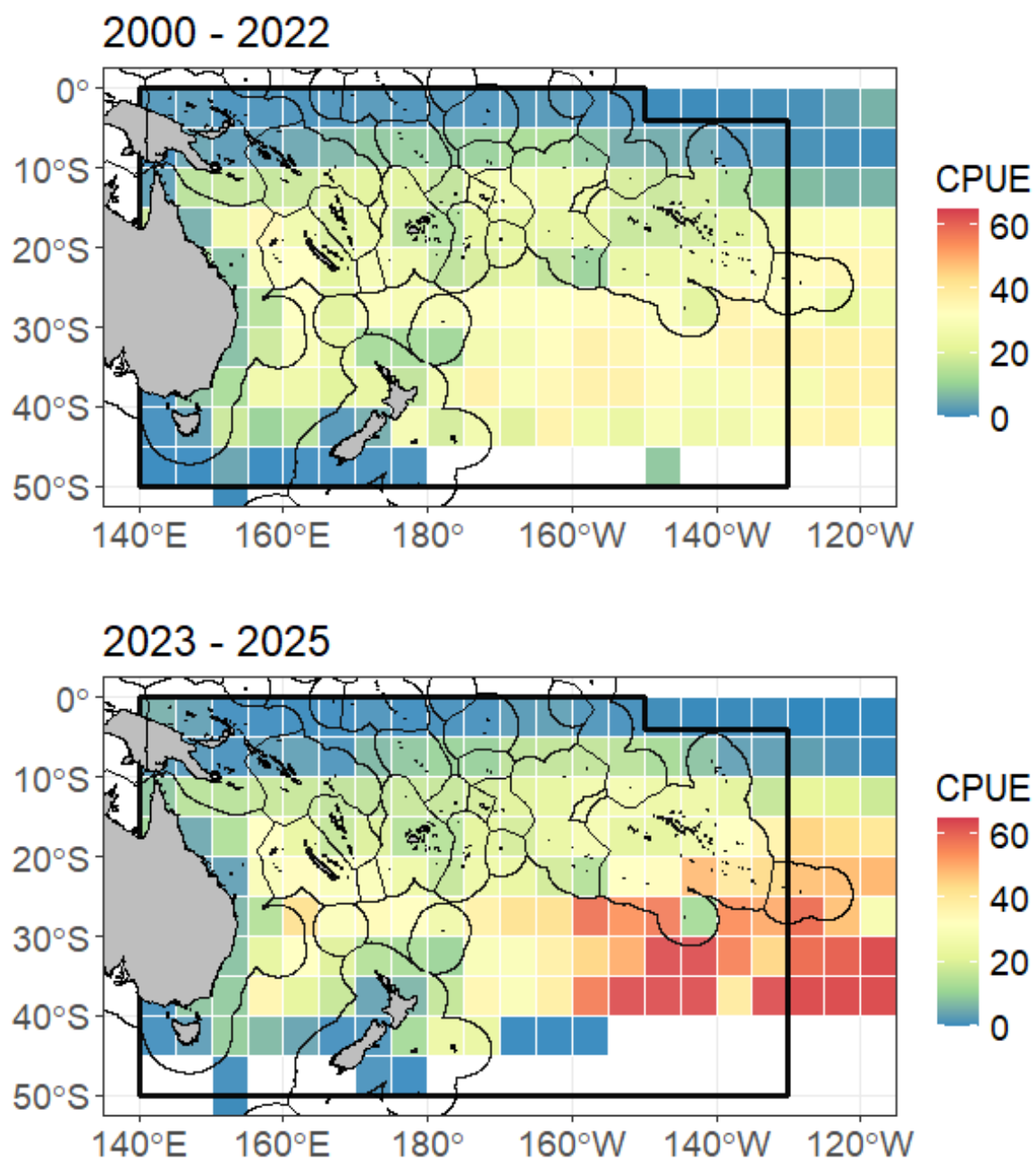
Figure 6: Albacore tuna longline CPUE distribution for the period 2000–2022 (top), and 2023–2025 (bottom). CPUE (kg/100 hooks) for a given 5^\circ \times 5^\circ square is indicated by the colour of the tile.
