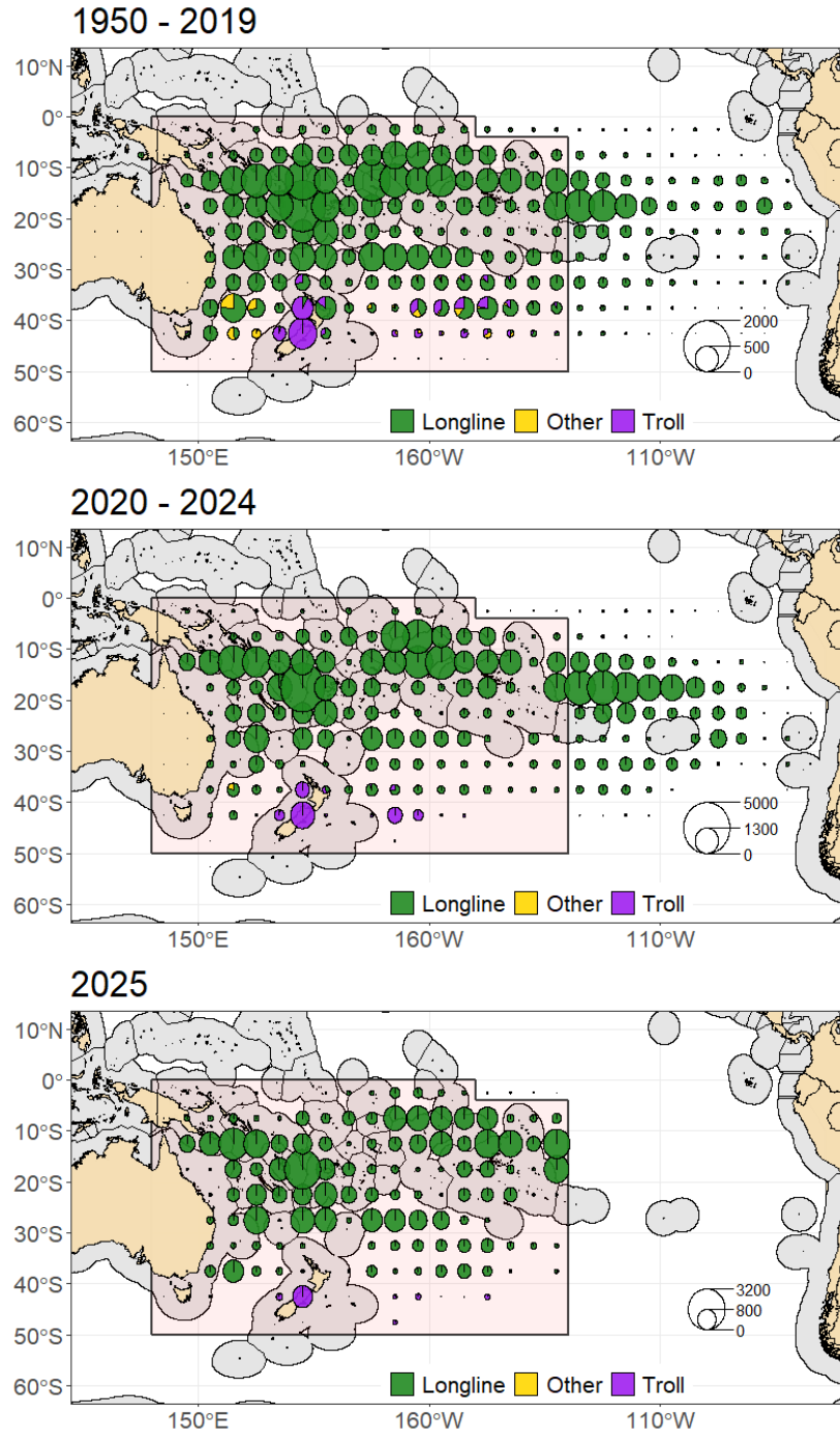
Figure 2: Albacore tuna catch distribution by gear type and 5°×5° degree region in the South Pacific Ocean for the period 1950-2019 (top), 2020 -2024 (middle) and 2025 (bottom). Circle size represents total catch volume with maximum circle size presented in the legends. Note that aggregate data for the EPO is not yet available for 2025.
