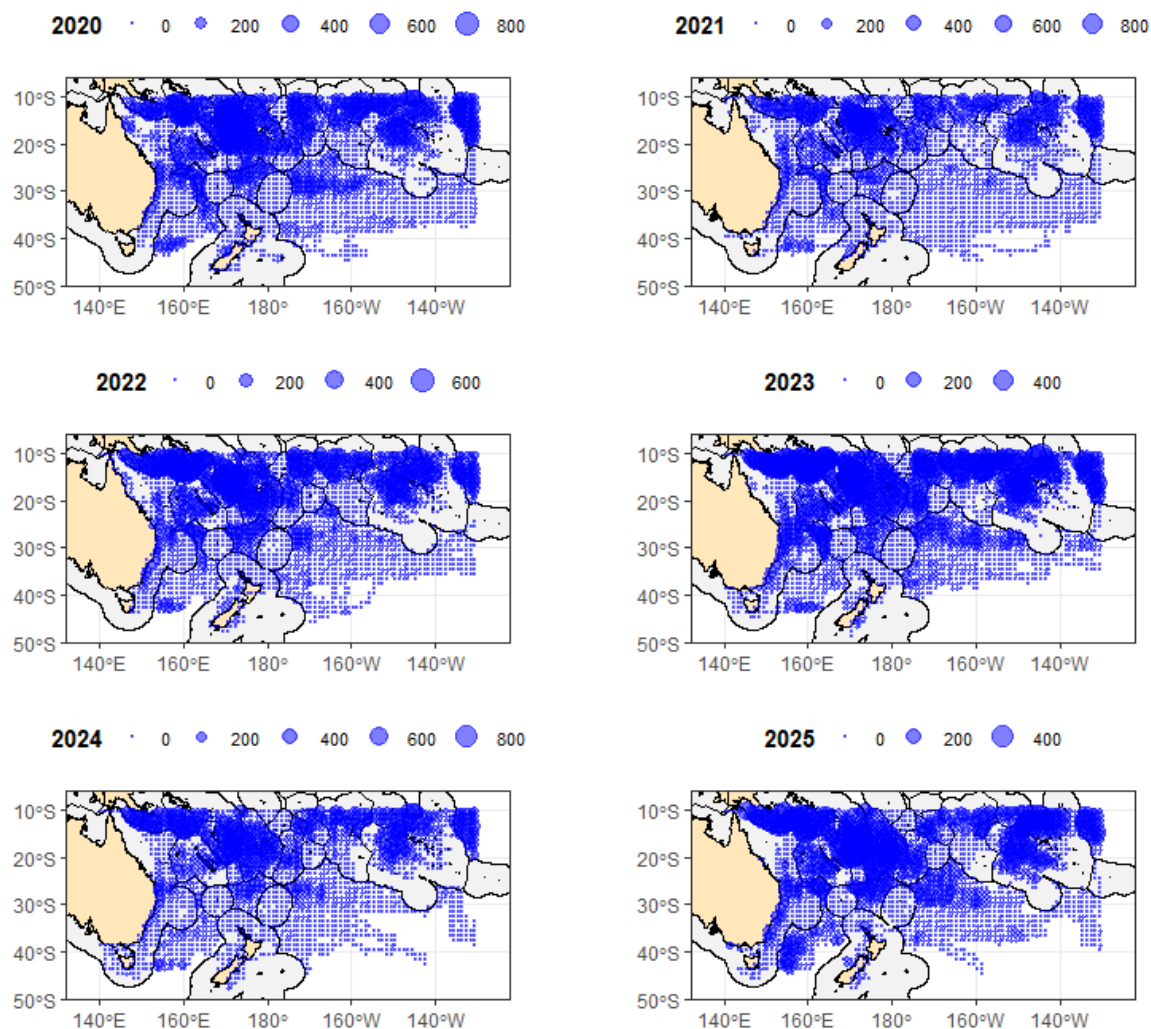
Figure 4: Longline VMS fishing days (augmented by logsheets for New Caledonia and French Polynesia) within the southern WCPFC-CA south of 10°S at the 1°x1° scale.
