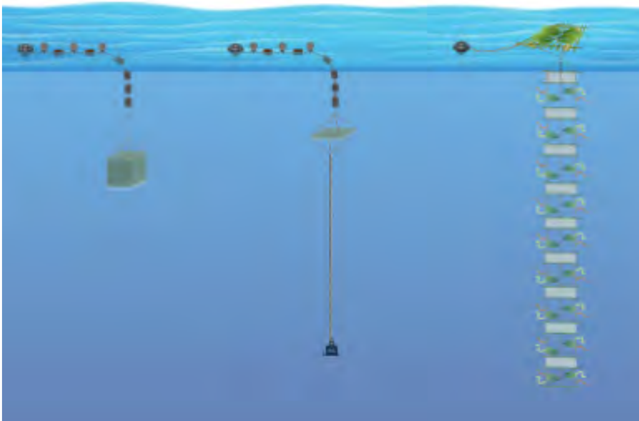
Figure 2. Schematic illustration of three representative conventional dFAD configurations: cage-type (left), tail-type (center), and curtain-type (right). Illustration courtesy of Albacora fishing company.
