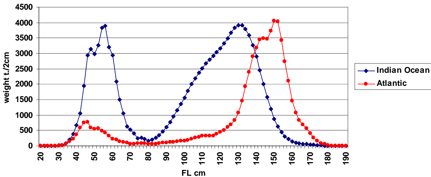
Average catches by 2 Cm class, YFT IO and Atlantic, Average 1997-2002
