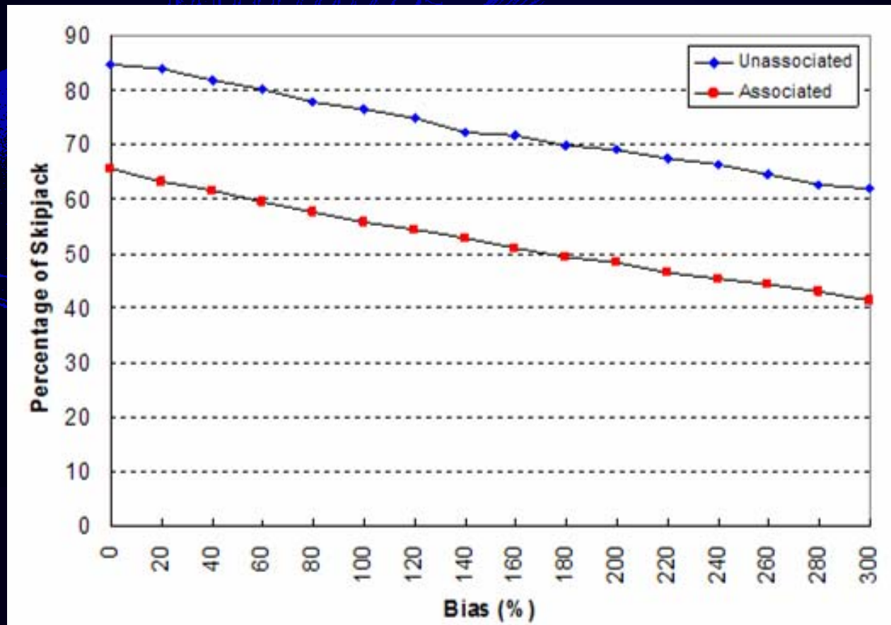
Figure 8. Relationship between bias in observer sampling and estimates of the percentage of skipjack in the catch, for simulated sampling of sets on an associated school and an unassociated school
