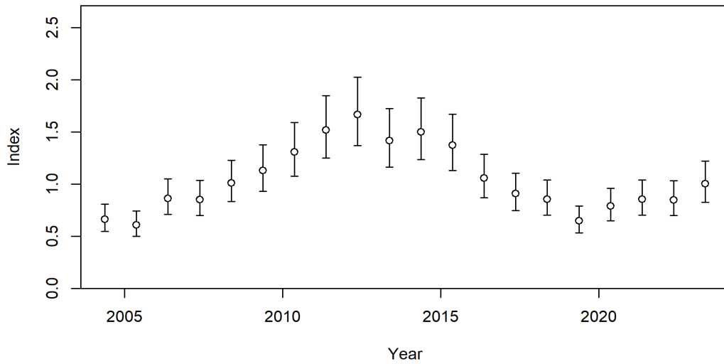
Figure SWO-04. Standardised CPUE with initial input 95% confidence interval (CI) for (top) the Australian longline CPUE index fishery in region 1 and (bottom) the New Zealand longline CPUE index fishery in region 2. Additional variance was estimated within the model, which effectively reduced these confidence intervals for the AU index and increased them for the NZ index.
