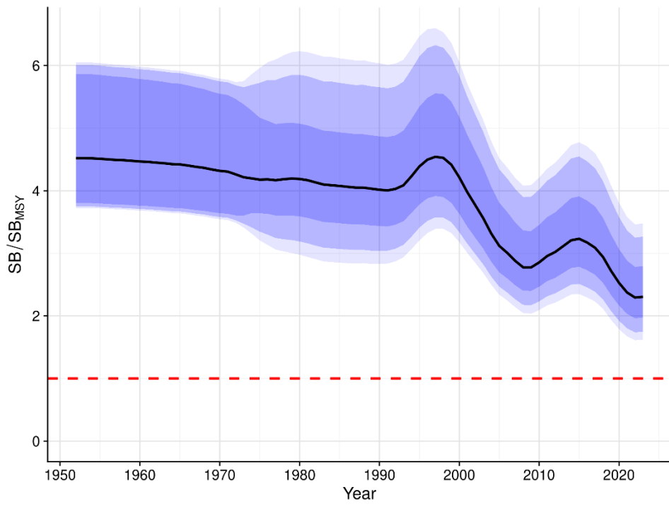
Figure SWO-08. Annual estimated F/F_{MSY} (top) and annual SB/SB_{MSY} (bottom) from the uncertainty grid. The black line indicates the median of all trajectories, along with 50%, 80% and 90% quantile ranges.
