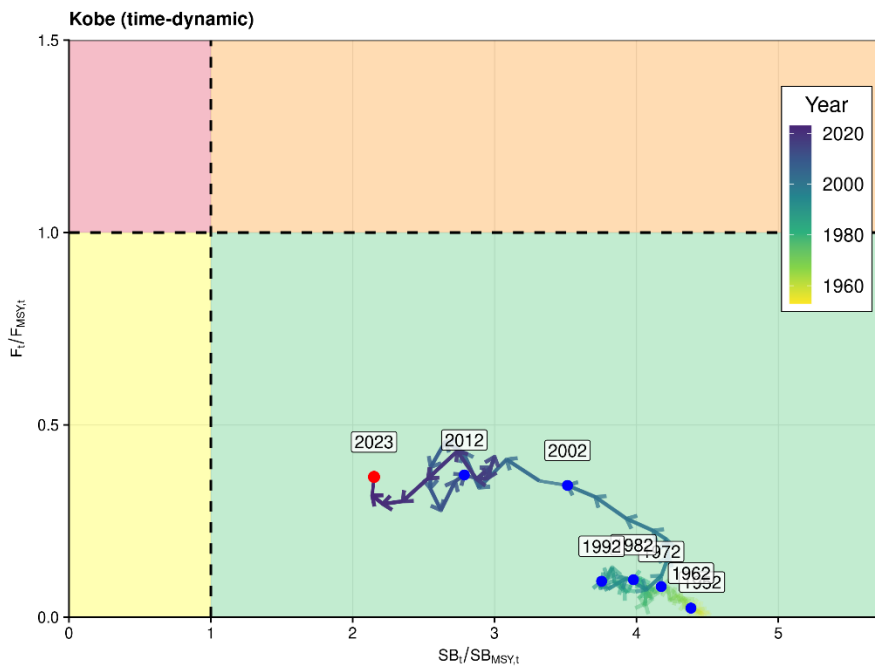
Figure SWO-12. Time dynamic Kobe plot from the diagnostic model for SWPO swordfish for the period 1952 to 2023 (red dot).
