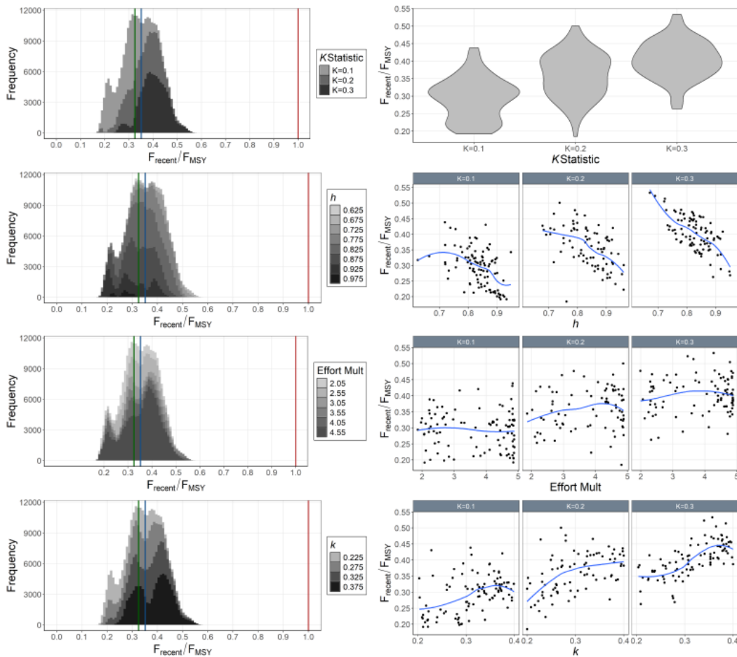
Figure SKJ-10. Histograms of Monte-Carlo estimated model uncertainty for F_{\text{recent}}/F_{\text{MSY}} by mixing period ( K statistic, top-left), h (2nd-left), effort multiplier (Effort Mult; 3rd-left), and growth coefficient k (bottom left) with mode (green line), median (blue line), and F_{\text{recent}}/F_{\text{MSY}} = 1.0 (red line). Also includes estimated F_{\text{recent}}/F_{\text{MSY}} by mixing period ( K statistic; top-right), h (2nd-right), effort multiplier (Effort Mult; 3rd-right), and growth coefficient k (bottom-right) for each model in the ensemble with a loess smoother.
