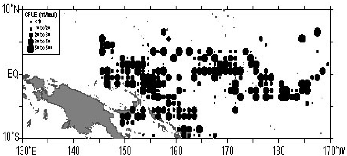
Fig. 5. Distribution of Korean tuna purse seine fishing area in the Pacific Ocean.
