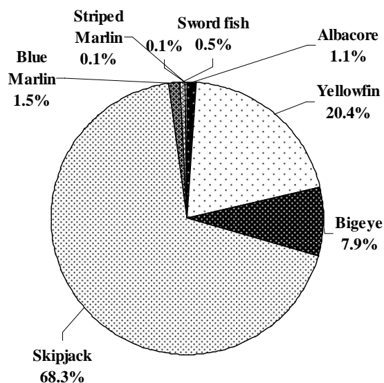
Fig. 1. Catch composition (averaged 2002-2006) of Korean tuna fisheries.
