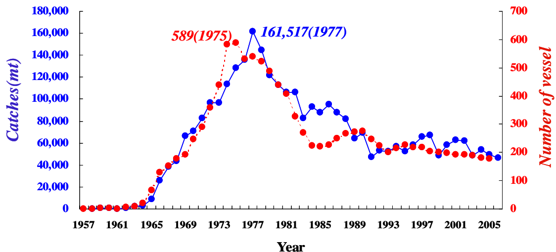
Fig. 3.. Annual catch and number of vessel of Korean tuna longline fisheries.
