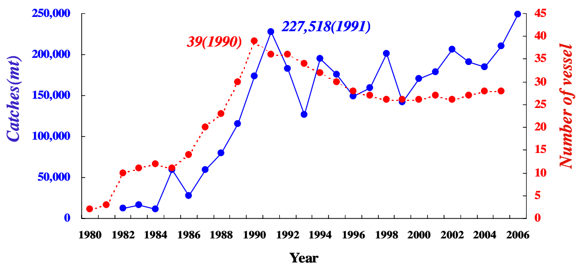
Fig. 2.. Annual catch and number of vessel of Korean tuna purse seine fisheries.
