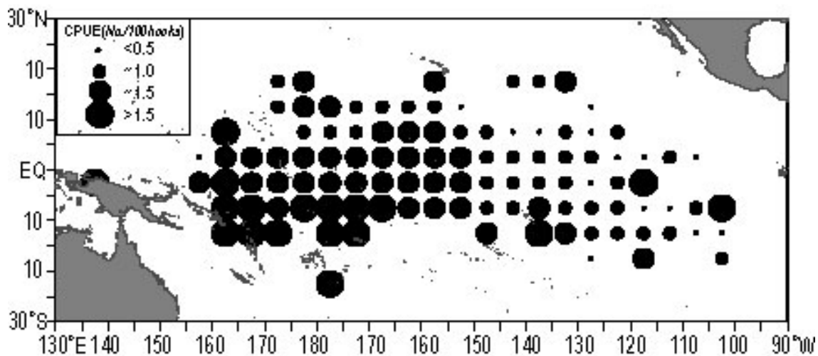
Fig. 6. Distribution of Korean tuna longline fishing area in the Pacific Ocean.
