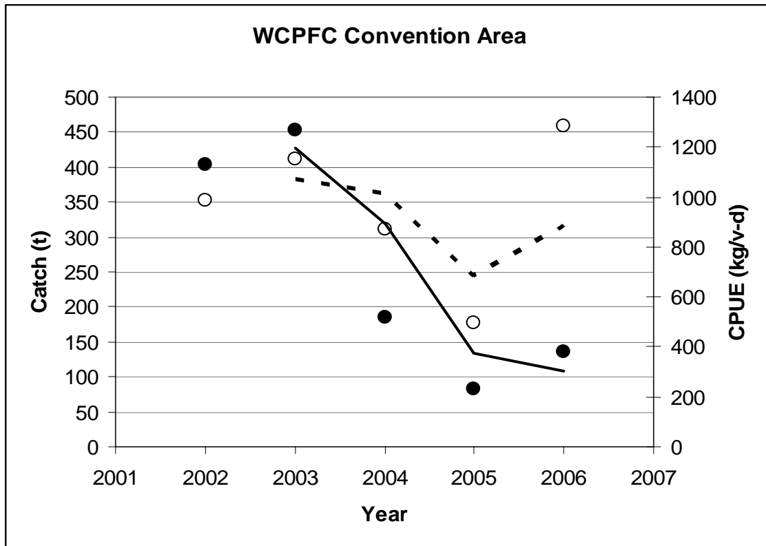
Figure 1. Canadian Pacific albacore catch (•) and CPUE (o) in the WCPFC convention area, 2002-2006.
