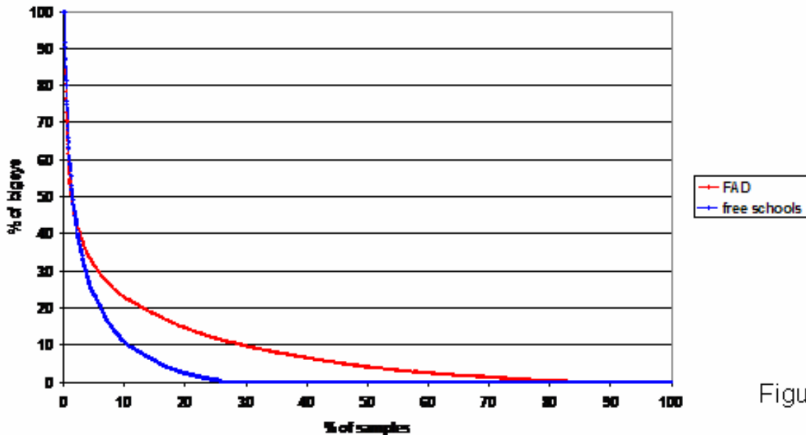
Figure 7: Percentages of bigeye (in weight) of in the FAD and in the free schools samples, classified by decreasing importance, observed in the Indian Ocean during the period 1990-2006 (the 5440 FAD and 3813 free schools samples being classified in the same scale of percentages) (figure taken from Fonteneau et al 2007)
