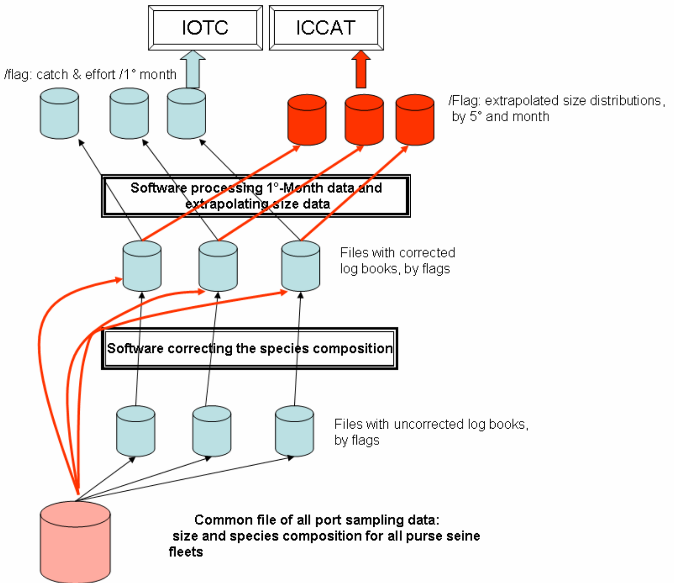
Figure 3: Conceptual organigram of the data processing of size and sampling composition of the EU purse seine data in the Atlantic and Indian oceans (since 1980)
