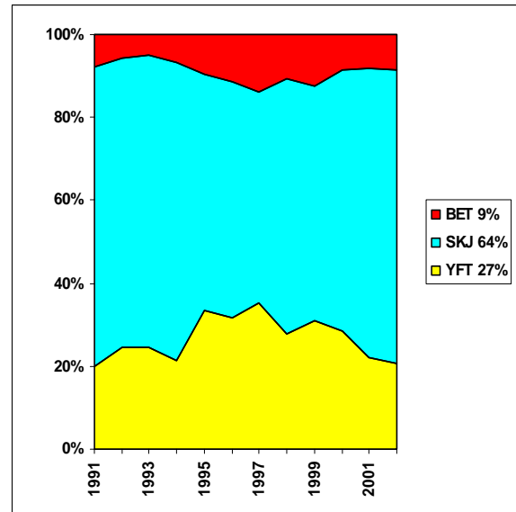
Figure 4: Species composition of FAD associated purse seine catches in the Indian Ocean as recorded in the log books and after correction of their species composition
