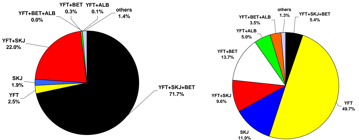
Figure 5: Average species composition of the FAD (5a) and Free schools (5b) samples and frequency of the various types of species composition observed in the Indian Ocean selected species samples (1990-2006) (figure taken from Fonteneau et al 2007)
