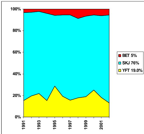
Figure 4: Species composition of FAD associated purse seine catches in the Indian Ocean as recorded in the log books and after correction of their species composition
