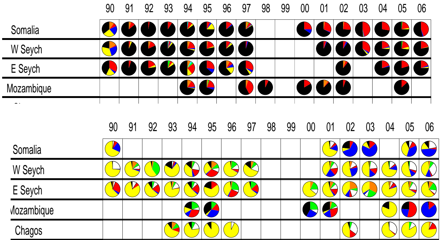
Figure 6: Frequency of species composition observed in the FADs (upper fig) and in the free schools samples (lower fig) expressed in % (only for strata with more than 10 samples each year) (figure taken from Fonteneau et al 2007)
