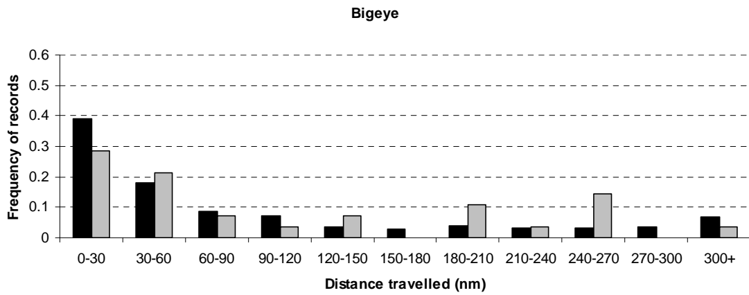
Figure 13 Frequency of distance between release and capture location for conventionally tagged skipjack, yellowfin and bigeye (Black bars= PNG releases and grey bars = Solomon Islands releases).
