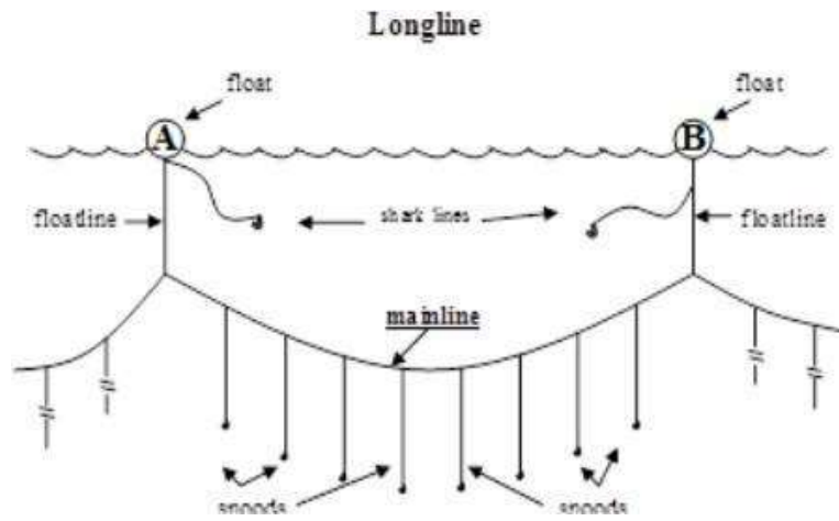
Annex 1: Schematic diagram of a shark line
