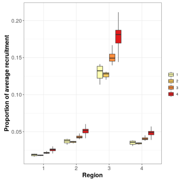
(c) 2021 SEAPODYM
